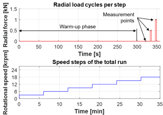
Figure 18. Test program.
