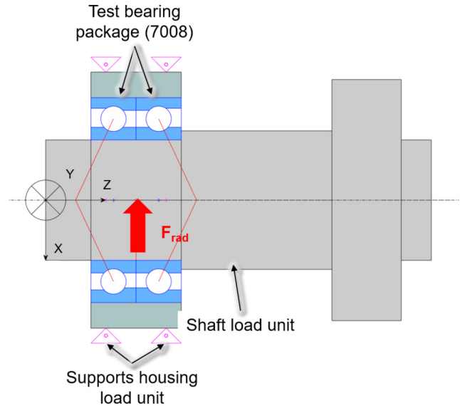
Figure 19. Simplified simulation model of the test rig.
