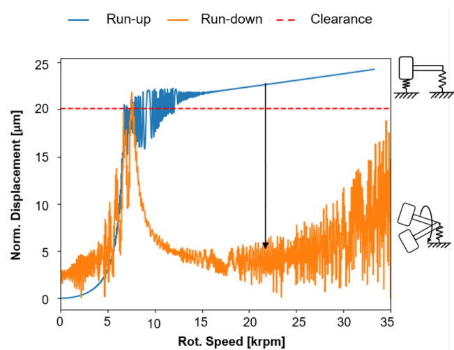
Figure 15. Supercritical operation of the cylindrical roller bearing (CRB).
