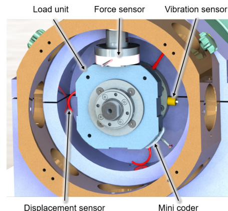
Figure 4. Load unit with sensors.
