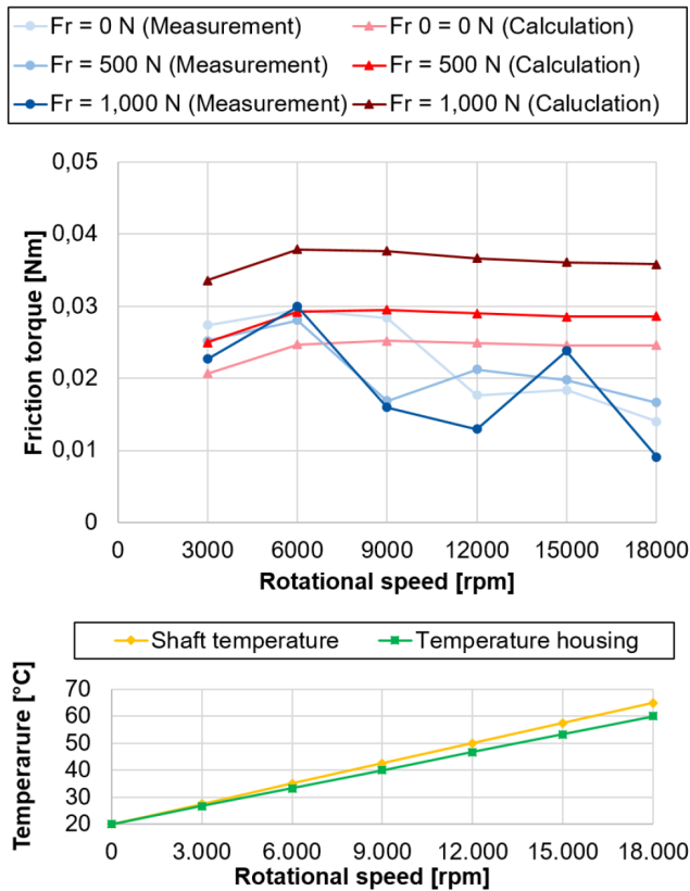
Figure 20. Comparison of measured and calculated bearing friction with temperature profiles. FR, radial load.
