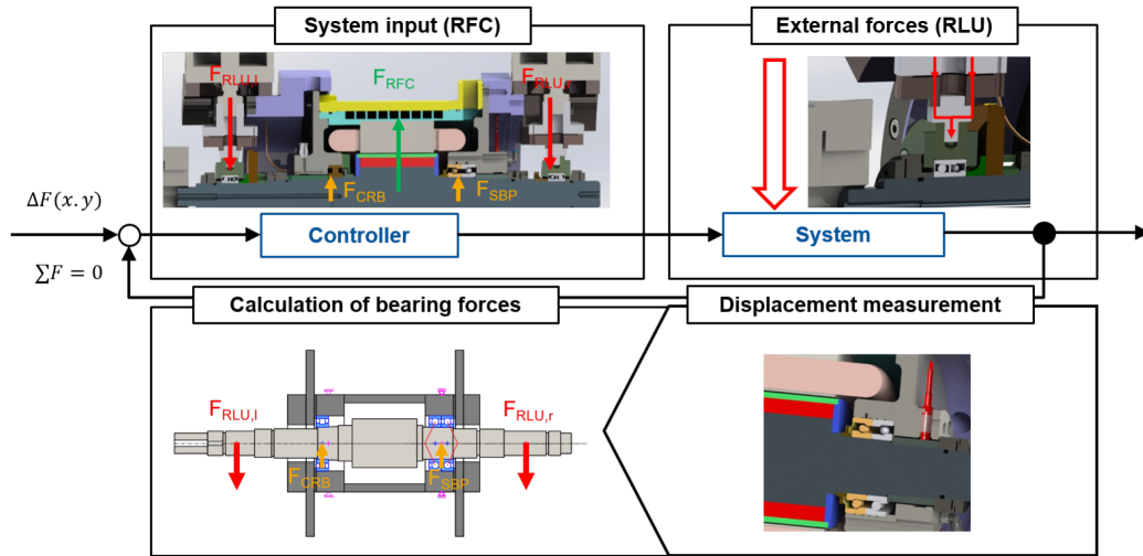
Figure 8. Simplified radial force control (RFC) loop. RLU, radial load unit; SBP, spindle bearing package; CRB, cylindrical roller bearing.
