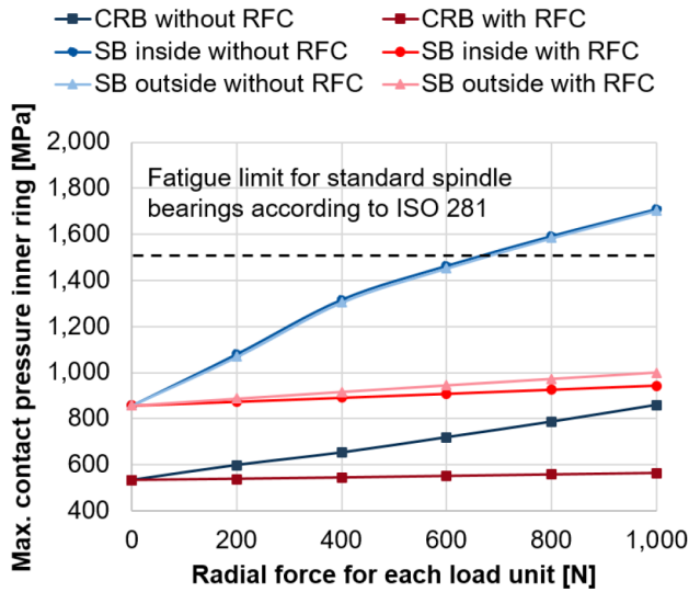
Figure 11. Maximum contact pressure on the inner ring. RFC, radial force control; CRB, cylindrical roller bearing; SB, spindle bearing.
