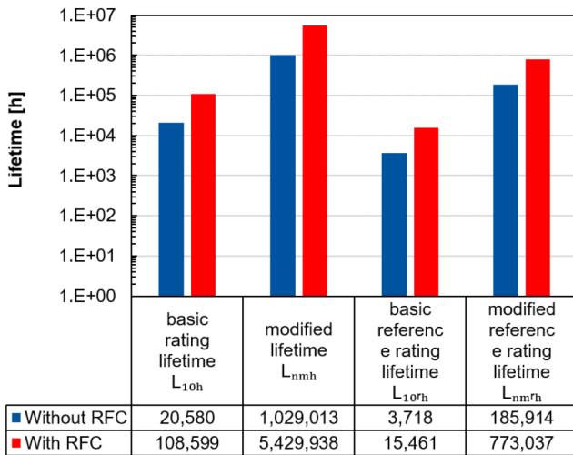
Figure 12. Lifetime calculation of the inside positioned spindle bearing with and without radial force control (RFC).
