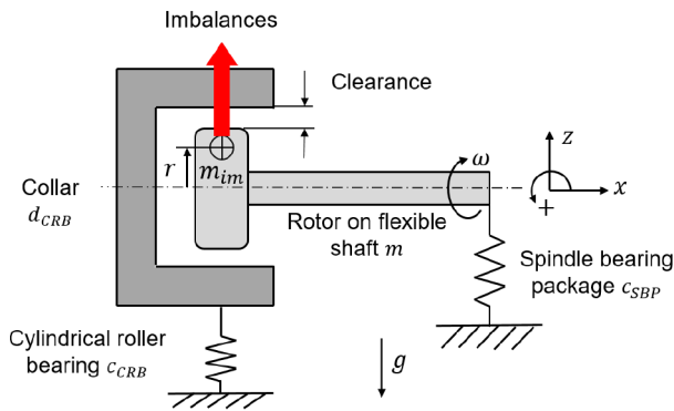
Figure 14. Shaft bearing system as spring mass damper.
