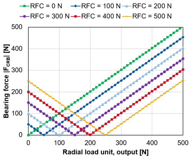
Figure 10. Variation of the generator radial force control (RFC). CRB, cylindrical roller bearing.
