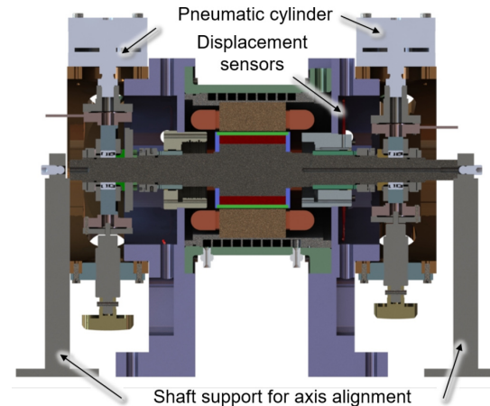
Figure 5. Cross section of the the calibration set up.
