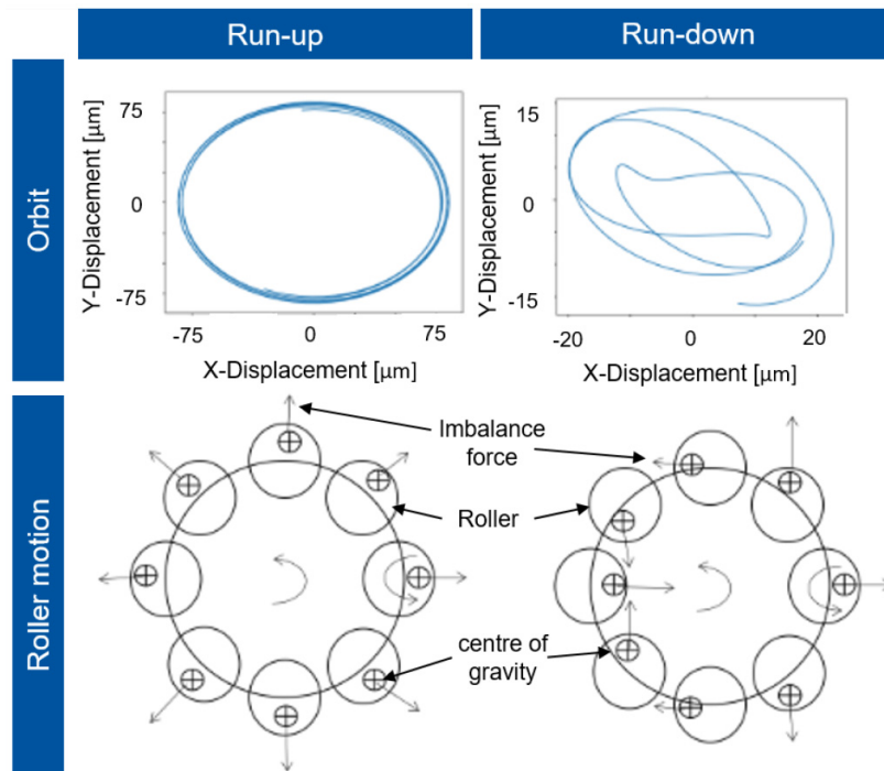
Figure 16. Shaft orbit and roller motion.
