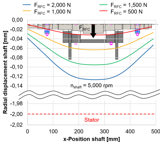
Figure 7. Radial shaft displacement (bearingless mode). RFC, radial force control.
