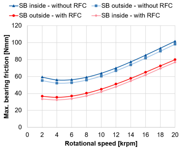
Figure 13. Maximum friction in the spindle bearings. RFC, radial force control; SB, spindle bearing.
