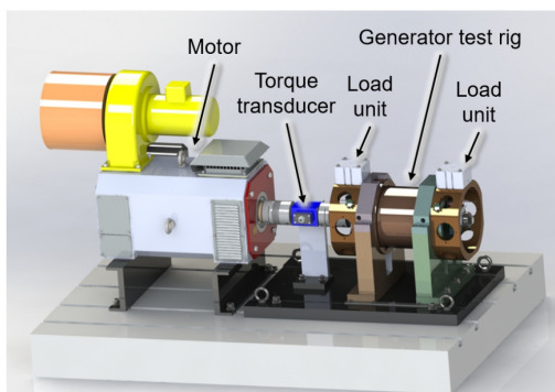
Figure 2. Generator test rig.
