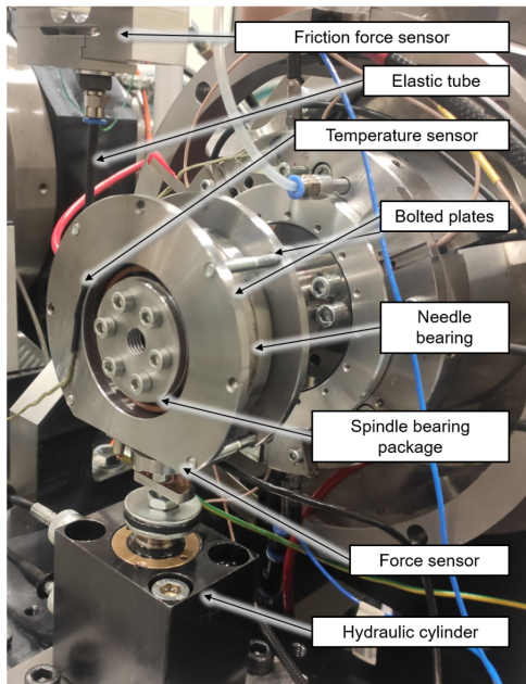
Figure 17. Radial load unit with friction measurement system.
