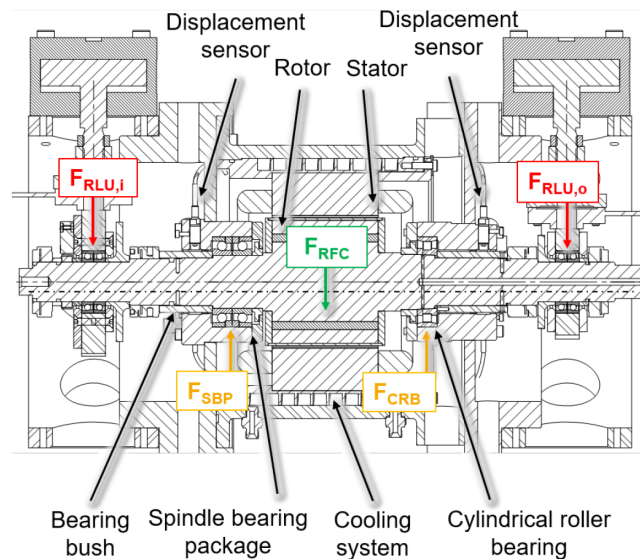
Figure 3. Cross section of the generator test rig. RFC, radial force control; RLU, radial load unit; SBP, spindle bearing package; CRB, cylindrical roller bearing.
