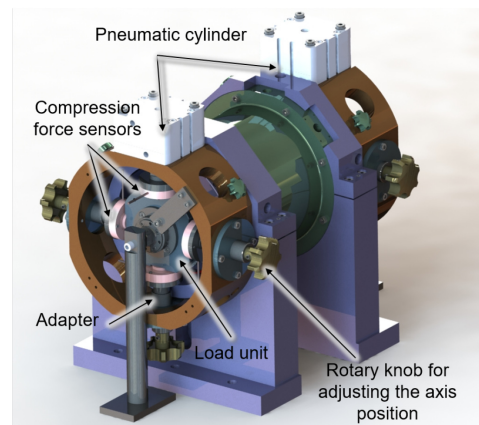
Figure 6. Set up of calibration measurement.
