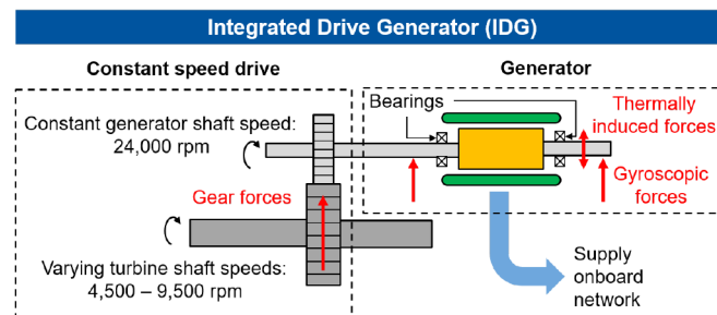
Figure 1. Schematic structure of the IDG (integrated drive generator).
