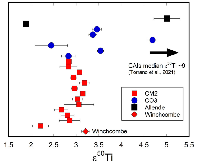
FIGURE 13. \epsilon^{50}\text{Ti} comparison between CM2 chondrites, CO3 chondrites, and Allende (CV3). See text for discussion. Data compiled from Trinquier et al. (2009), Zhang et al. (2011, 2012), Torrano et al. (2021), this study.
