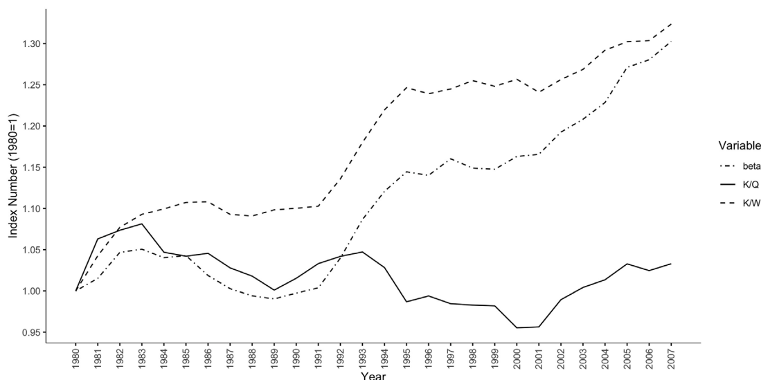
Fig. 1. Dynamics of fixed capital to wages (K/W), fixed capital to net output (K/Q) and \beta (beta) for Italy (1980–2007).
