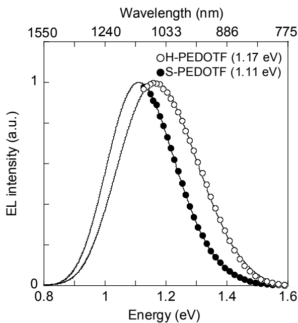
FIGURE 3 CT EL spectra from the BHJ layers of H-PEDOTF:PC 70 BM and S-PEDOTF:PC 70 BM (1:4). The values shown in parentheses are the energies of CT EL peaks. The solid lines are Gaussian fitted curves of obtained CT EL spectra.
