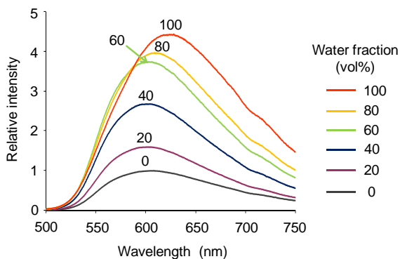
Fig. 3. Emission spectra of 2 in methanol/water mixtures ( 5 \times 10^{-5} M, \lambda_{ex} = 385 nm).
