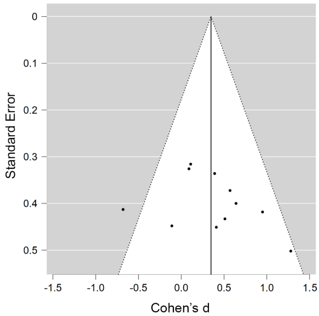
Figure 27. Funnel plot for the TUG test outcome.
