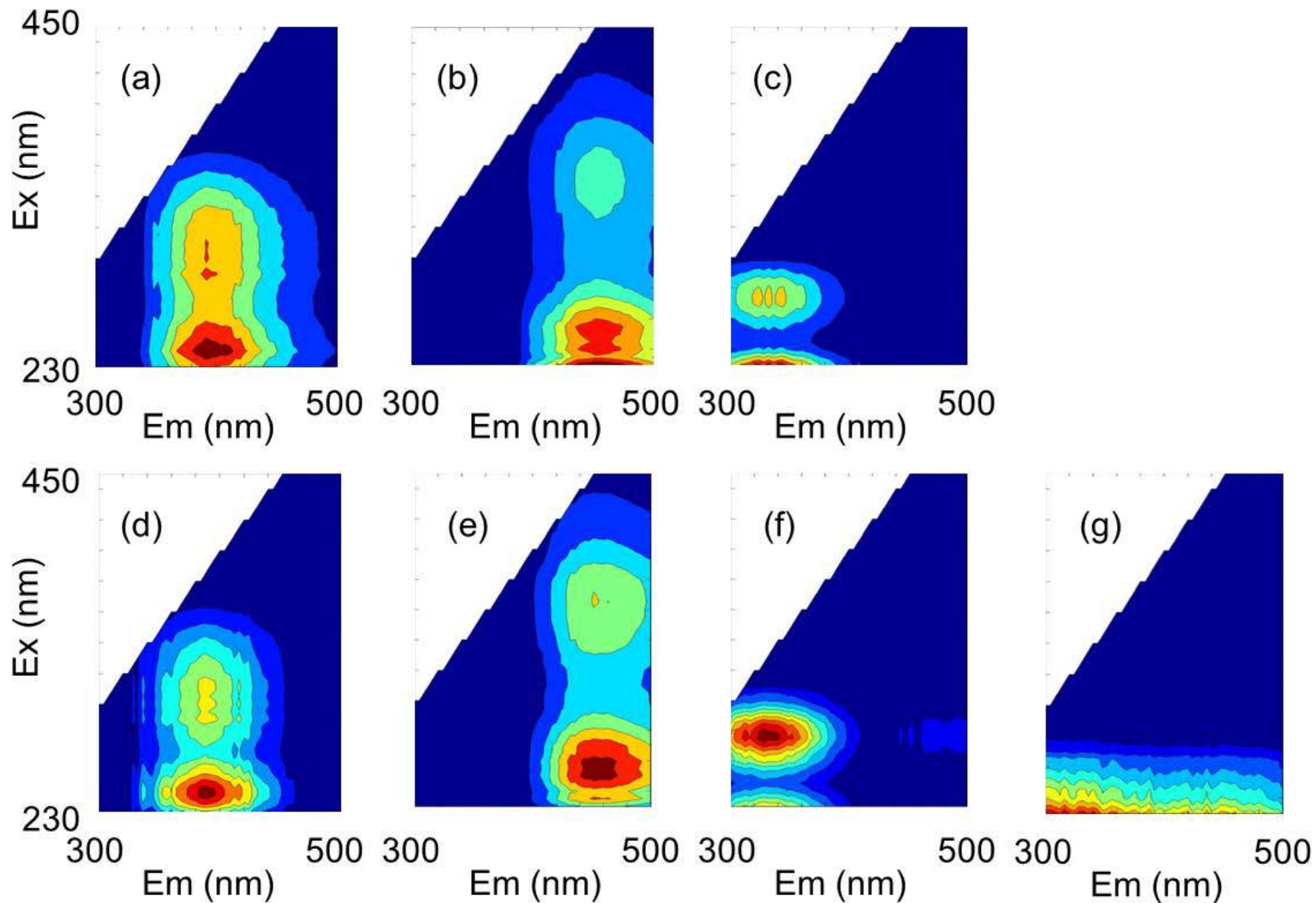
Fig. 3 Fluorescent components identified by PARAFAC analysis.
