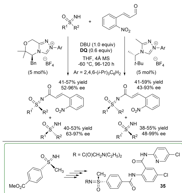
Scheme 41. NHC-catalyzed KR of sulfoximines via oxidative amidation.
