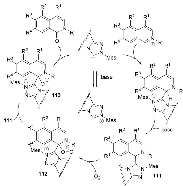
Scheme 93. NHC-catalyzed aerobic oxidation of isoquinolinium/phenanthridinium salts.
