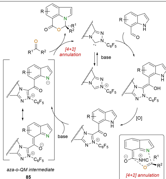
Scheme 79. Annulation of indole-7-carboxaldehydes with ketones via NHC-bound aza-o-QM intermediate.
