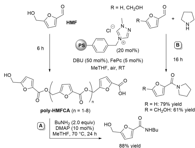
Scheme 44. One-pot two-step approach to HMFCAs amide (A) and direct amidation of HMF/FF (B) via aerobic oxidative NHC-catalysis.
