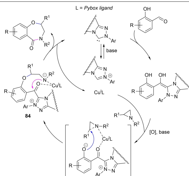
Scheme 78. Synthesis of 1,4-benzoxazepinones via NHC-bound o -QM intermediate under copper (I) co-catalysis.
