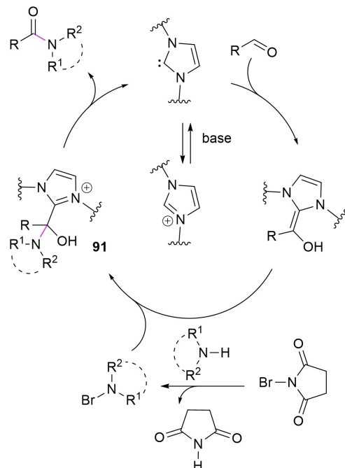
Scheme 84. NHC-catalyzed oxidative amidation of aldehydes with amines promoted by NBS.
