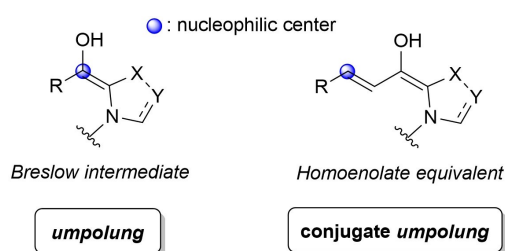
Figure 1. Typical umpolung reactivity of NHCs.
