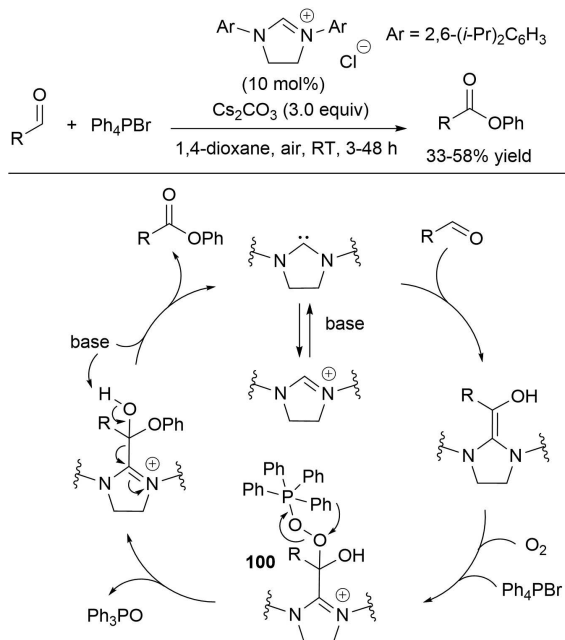
Scheme 89. NHC-catalyzed aerobic oxidative esterification of aldehydes with Ph 4 PBr.
