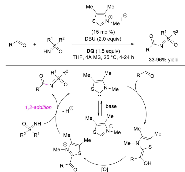
Scheme 42. Oxidative N -acylation of sulfoximines by NHC-catalysis.
