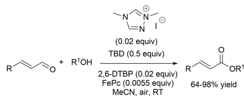
Scheme 26. Aerobic oxidative esterification of enals with alcohols by NHC/ETMs system.
