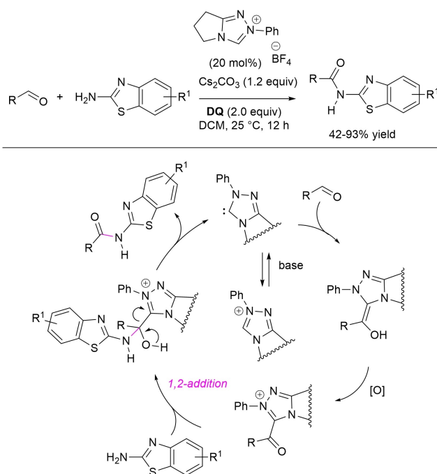
Scheme 34. Direct oxidative amidation of aldehydes with 2-aminobenzothiazoles.
