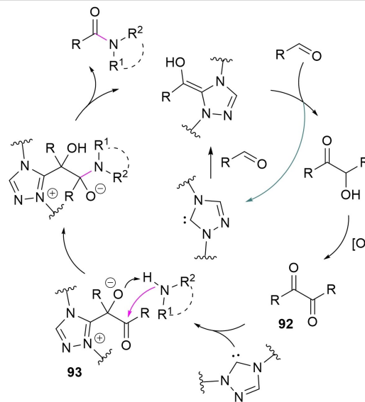
Scheme 85. NHC-catalyzed oxidative amidation of aldehydes with amines promoted by PHZ.
