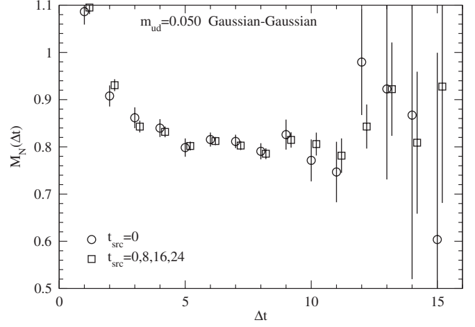
FIG. 6. Improving the statistics by averaging the nucleon two-point functions calculated from four different source points at time slices t_{\text{src}} = 0, 8, 16, \text{ and } 24 . The result for M_N(\Delta t) (squares) is compared with that without the average, i.e., t_{\text{src}} = 0 . The quark mass is m_{ud} = 0.050 . The Gaussian smearing is used for both the nucleon source and sink.
