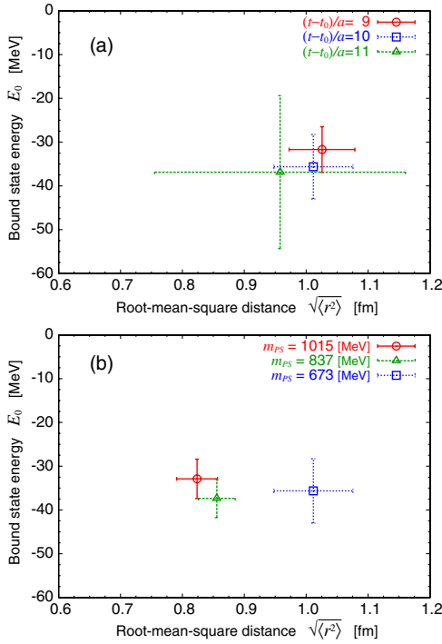
FIG. 3 (color online). Bound state energy E_0 \equiv -\tilde{B}_H and the rms distance \sqrt{\langle r^2 \rangle} of the H dibaryon obtained from the potential at L = 3.87 fm. (a) Imaginary-time dependence at m_{ps} = 673 MeV. (b) Quark mass dependence at (t - t_0)/a = 10 .
