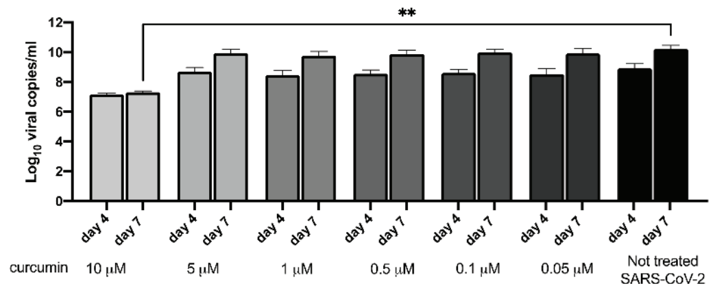
Figure 2. Effect of different concentrations of curcumin (10, 5, 1, 0.5, 0.1, and 0.05 \mu\text{M} ) on SARS-CoV-2 viral load on days 4 and 7 post-treatment/infection. The viral load is expressed as Log 10 viral copies/mL. Result from Kruskal–Wallis tests, adjusted for Dunn’s multiple comparisons test, are displayed. ** p -value < 0.01.
