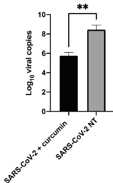
Figure 3. The effect of curcumin (10 \mu\text{M} ) on virion integrity, tested by means of the RNase protection assay. Non-treated (designed as SARS-CoV-2 NT) and treated viruses (designed as SARS-CoV-2 + curcumin) are displayed. The viral load is expressed as Log 10 viral copies. Results from Mann–Whitney tests are shown. ** p -value < 0.01.
