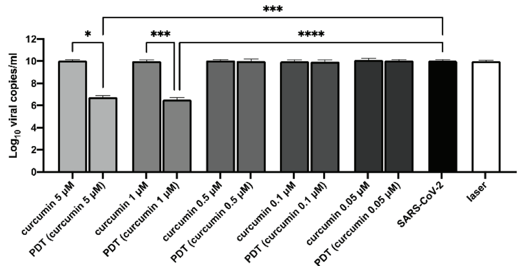
Figure 4. Results of photodynamic treatment (PDT) with different concentrations of curcumin (5, 1, 0.5, 0.1, and 0.05 \mu\text{M} ) on SARS-CoV-2 infectivity (viral load) on day 7 post-treatment/infection. The data obtained through the irradiation of the virus without curcumin (indicated as “laser” in the figure), the treatment of the virus with curcumin without irradiation (designed as “curcumin”), and the non-treated virus (not irradiated and not challenged with curcumin, indicated in the figure as “SARS-CoV-2”) are also reported. The viral load is expressed as Log 10 viral copies for mL. Results of Kruskal–Wallis test, adjusted for Dunn’s multiple comparisons test, are displayed. **** p -value < 0.0001 ; *** p -value < 0.001 ; * p -value < 0.05 .
