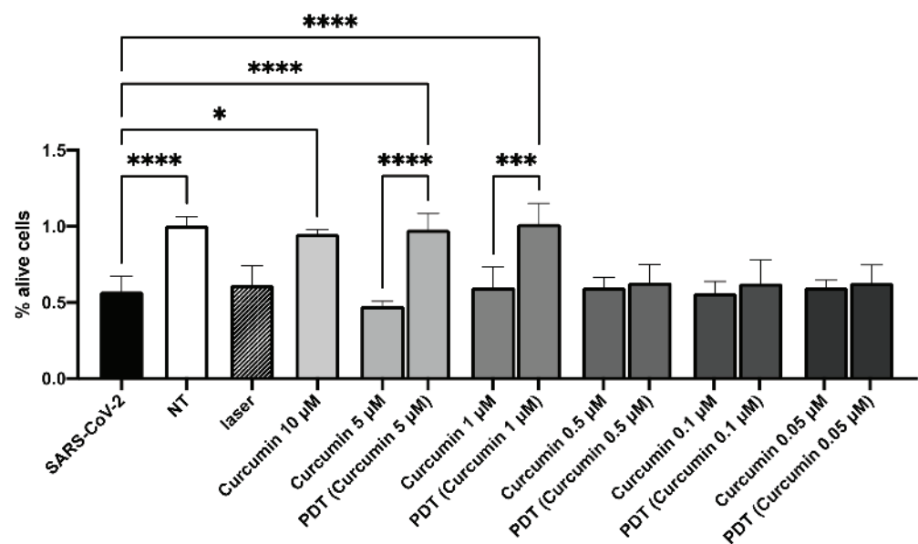
Figure 5. Viability at 7 days of the cells inoculated with curcumin-treated virus (indicated as 2curcumin”), PDT-treated virus (indicated as “PDT curcumin”), or untreated virus (indicated as “SARS-CoV-2”). Non-infected cells (indicated as NT) and cells infected with irradiated virus without curcumin (indicated as “laser”) are also shown. The data are presented as a percentage of living cells relative to the non-treated cells (NT). Results from Kruskal–Wallis test, adjusted for Dunn’s multiple comparisons test, are displayed. **** p -value < 0.0001; *** p -value < 0.001; * p -value < 0.05.
