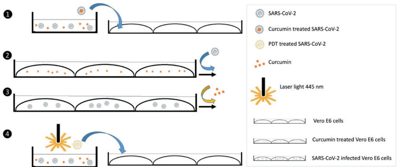
Figure 1. A graphical representation of the experimental settings employed: (1) the incubation of the virus with curcumin prior to its inoculation on cell culture (2) curcumin prophylactic treatment of cells (3) curcumin treatment of SARS-CoV-2 infected cells (4) curcumin based photodynamic treatment of SARS-CoV-2.
