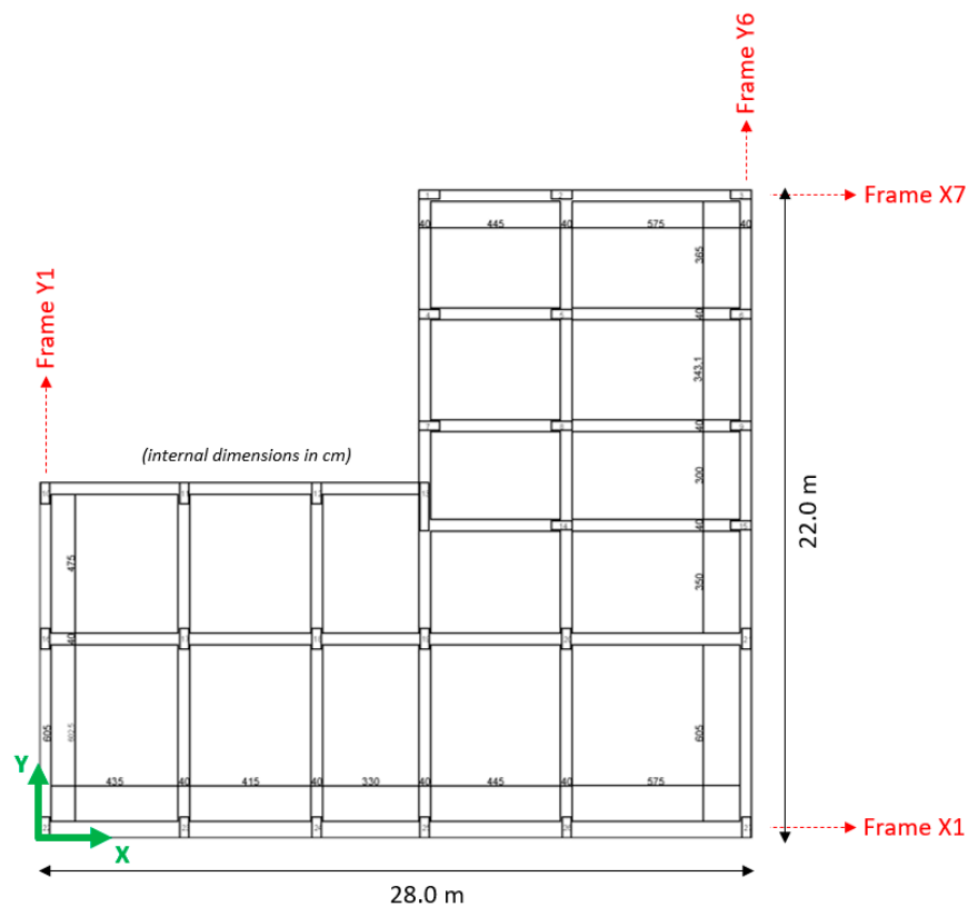
Figure 2. Typical horizontal section of the 1st floor (scanned archive drawings).
