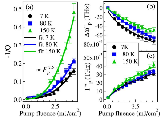
FIG. 2. (Color online) (a) The Fano parameter -1/Q , (b) the frequency shift \Delta\omega_p'' , and (c) the broadening \Gamma_p'' as a function of F_p at various temperatures. The data extracted from the low excitation intensity data (measured at F_p=9.2 \text{ } \mu\text{J/cm}^2 ) are also plotted. The solid curves in (a) are the fitting with F_p^{2.5} , while the solid curves in (b) and (c) show F_p^\theta behavior with 0.5 < \theta < 0.8 (see text).
