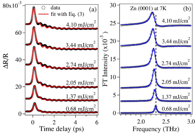
FIG. 1. (Color online) (a) Transient reflectivity change obtained in Zn at T_l=7 K at various pump fluences and (b) their FT spectra. In both panels, open circles are the experimental data, while solid lines present fits with Eqs. (3) and (1), respectively.
