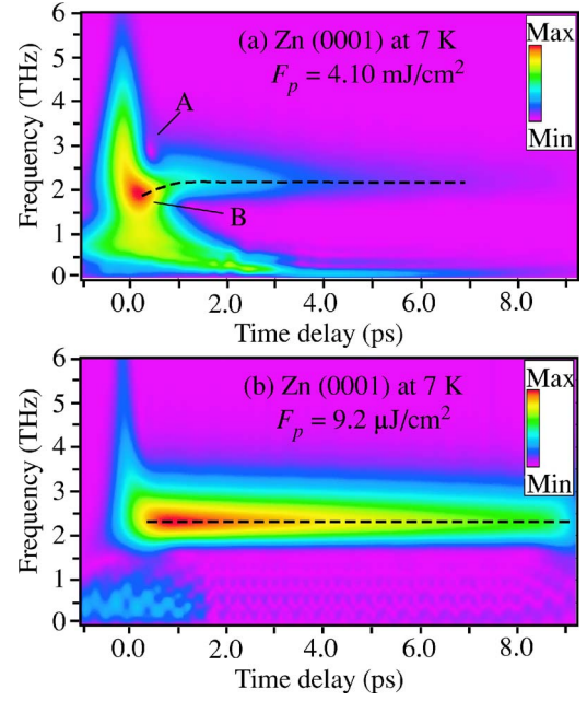
FIG. 3. (Color online) CWT chronograms in Zn at 7 K for two different pump fluences, (a) 4.1 \text{ mJ}/\text{cm}^2 and (b) 9.2 \mu\text{J}/\text{cm}^2 . The broad band response extending below 1 THz up to 6 THz and decaying within a few ps in (a) represents the transient response that is due to inter- and intraband electronic Raman scattering, while the dotted curves represent the peak positions of the coherent E_{2g} phonon.
