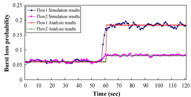
Fig. 7. Burst loss probability in single congested link system with RFP-A implementation.
