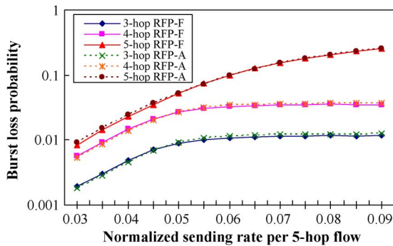
Fig. 10. Burst loss probability in RFP-F-based and RFP-A-based NSF networks.
