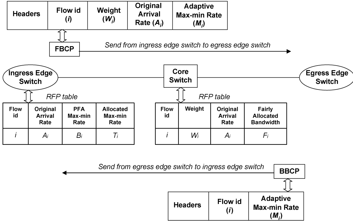
Fig. 1. Parameters contained in FBCP, BBCP, and RFP table of edge and core switches.
