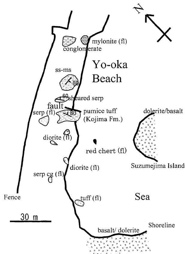
Fig. 9 Lithology map of the Yo-oka Beach. Adopted from Ogawa and Sashida (2006) with some revisions.
