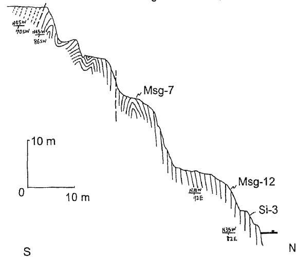
Fig. 14 Cross section of the alternations of chert and limestone beds at Shiraginu Waterfall, north of Mineoka-Sengen.
