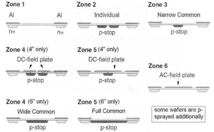
Fig. 1. Electrical strip isolation structures, Z1 to Z6, implemented for 4" and 6" processes. The field plates for Z4 to Z6 are poly-silicon. The structures with DC field plates Z4 and Z5 in 4" are modified to wider and full wide p-stop in 6". Three p-stop concentrations were examined with p-spray added to the lowest concentration.
