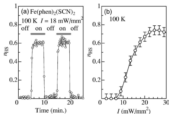
FIG. 1. (a) On-off optical switching of the density of the high-spin species ( n_{\text{HS}} ) measured at 100 K. The gray horizontal bar represents the on-off action of the excitation light at 532 nm. (b) Excitation power density ( I ) dependence of n_{\text{HS}} in the “on phase” at 100 K.
