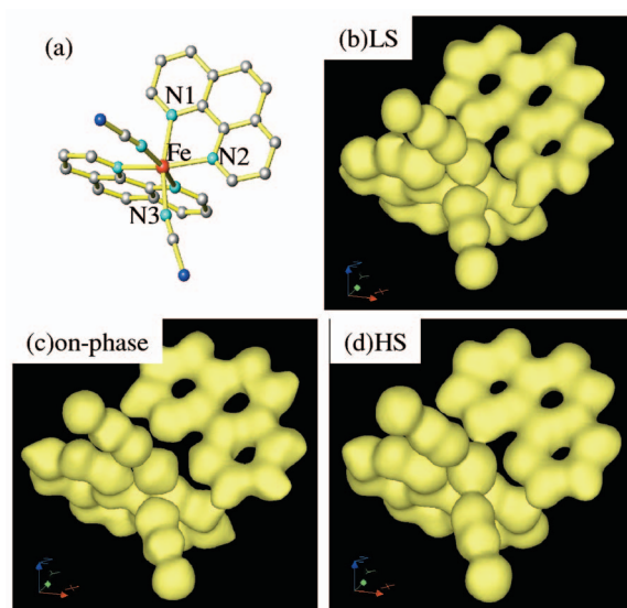
FIG. 4. (Color) (a) Ball and stick picture of the \text{Fe}(\text{phen})_2(\text{NCS})_2 molecule. Isodensity surface contour ( 0.45 \text{ \AA}^{-3} ) of the \text{Fe}(\text{phen})_2(\text{NCS})_2 molecule in (b) the LS phase at 92 K, (c) the on phase at 92 K, and (d) the HS phase at 260 K, determined by the MEM/Rietveld analysis.
