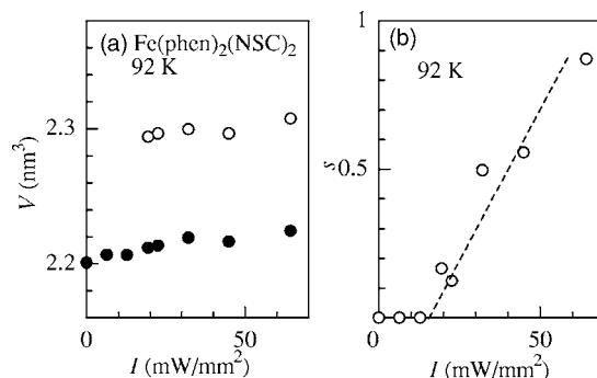
FIG. 3. (a) Cell volume ( V ) of \text{Fe}(\text{phen})_2(\text{NCS})_2 at 92 K against excitation power density ( I ). Closed and open circles stand for the LS phase and the on phase, respectively. (b) Mass fraction ( s ) of the on phase against I . A broken straight line is merely the guide for the eyes.
