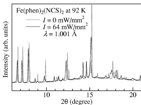
FIG. 2. X-ray powder diffraction patterns of \text{Fe}(\text{phen})_2(\text{NCS})_2 at 92 K under photoexcitation ( I=64 \text{ mW/mm}^2 ; black curve) and without photoexcitation (gray curve).
