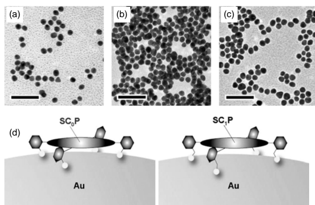
Figure 1. TEM images of (a) citrate- (b) SC_0P - and (c) SC_1P -protected Au nanoparticles. Particle diameters are (a) 10.5 \pm 1.0 nm, (b) 10.5 \pm 1.0 nm and (c) 10.0 \pm 0.9 nm, respectively. Scale bar indicates 50 nm. (d) Schematic illustrations of the coordination of SC_nP ligands on the Au surface.
