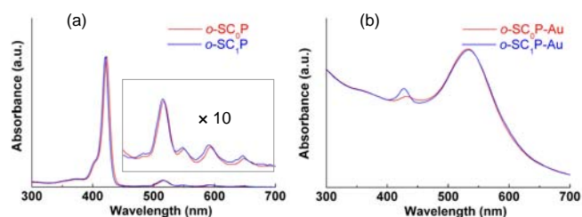
Figure 3. UV-Vis spectra of (a) SC n P ligands and (b) SC n P-Au nanoparticles. Inset in (a) shows the Q-bands expanded by 10. Each set of spectra was normalized by (a) ligand and (b) nanoparticle concentrations.
