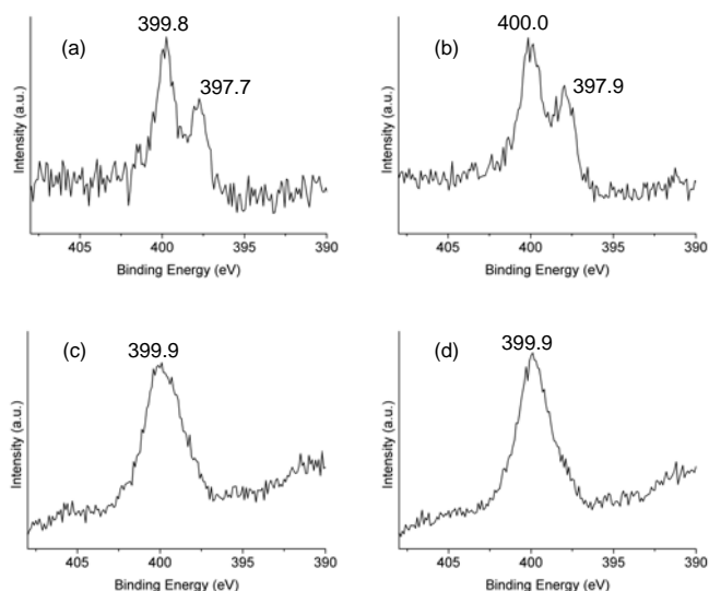
Figure 2. N1s core level XPS spectra for (a) SC 0 P, (b) SC 1 P, (c) SC 0 P-Au and (d) SC 1 P-Au
