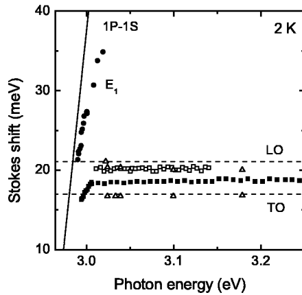
FIG. 2. Stokes shifts of the satellite holes E_1 (solid circles) and LO (solid squares) in CuBr QD's in glass as a function of photon energy of the satellite holes. The solid line shows the size dependence of the energy difference between exciton states 1S and 1P . The dashed lines represent the energies of LO and TO phonons in a bulk CuBr crystal, respectively. The open squares and triangles show the energies of LO and TO phonons in CuBr QD's in glass, which were measured by Raman scattering (Refs. 19–22).
