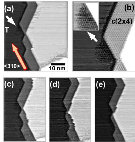
FIG. 3 (color online). (a), (c)–(e) show a sequence of STM images obtained every 512 sec; (b) shows a magnification of the area indicated by the arrow T in (a). The inset in (b) is a high-contrast image of the triangular structure.
