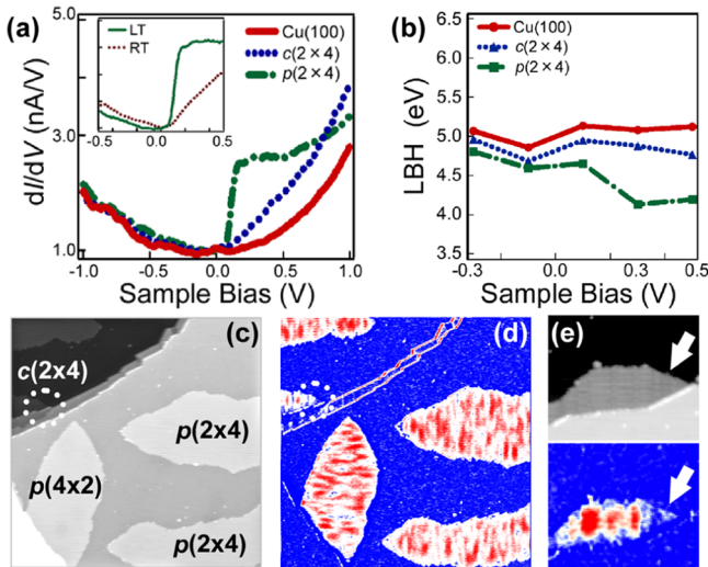
FIG. 4 (color online). (a) Spectra obtained at 5 K. (b) LBH spectra obtained at 5 K (set point: 1 M \Omega , 0.1 nA, 0.1 V). Data were obtained by measuring the I - Z curve as the STM tip was retracted 0.3 nm from the set point; (c), (d) show topographic and dI/dV images of a glycine-deposited surface (200 nm \times 200 nm, +0.11 V, 1.2 nA), and (e) shows magnified topographic and dI/dV images, where c(2 \times 4) triangular (indicated by white arrow) and neighboring p(2 \times 4) structures coexist (+0.13 V, 0.2 nA).
