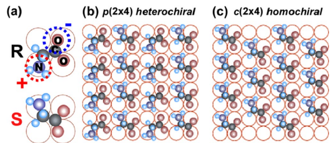
FIG. 1 (color online). (a) Two conformations of an adsorbed glycine molecule, and molecular arrangements of (b) p(2 \times 4) and (c) c(2 \times 4) structures.
