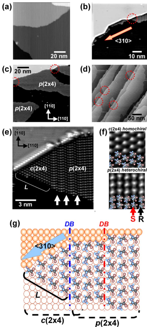
FIG. 2 (color online). STM images obtained at 5 K for the bare (a) and glycine-deposited Cu(100) surfaces (b) 0.2, (c) 0.4, and (d) 0.6 ML. (e) A magnified STM image of the area indicated by red circles in (b)–(d). (f) Magnifications of c(2 \times 4) and p(2 \times 4) areas with molecular arrangements, (g) Structural models of the molecular arrangements in (e).
