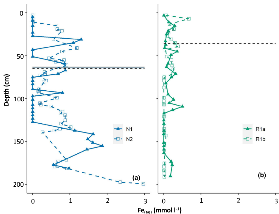
FIGURE 4 Aqueous iron (Fe (aq) ) with depth in cores (a) N1 and N2, and (b) R1a and R1b. The horizontal dashed line in (a) shows the thaw depth in N2 at the end of summer 2017, whereas the solid horizontal line shows the thaw depth in N1 at the end of summer 2017. The horizontal dashed line in (b) shows the thaw depth in R1 at the end of summer 2017. [Colour figure can be viewed at wileyonlinelibrary.com ]
