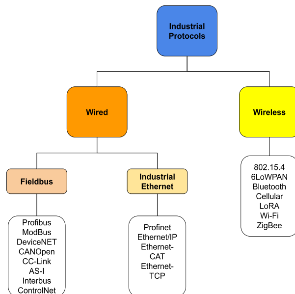
FIGURE 6. Industrial protocols for data transmission.
