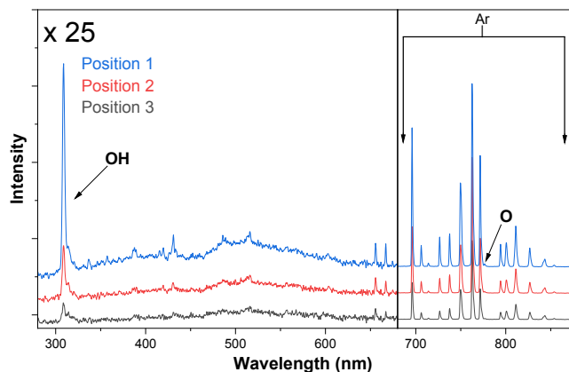
Figure 4 OES measurements of plasma glow in contact with water at positions 1, 2, and 3 as marked on Fig. 1.
