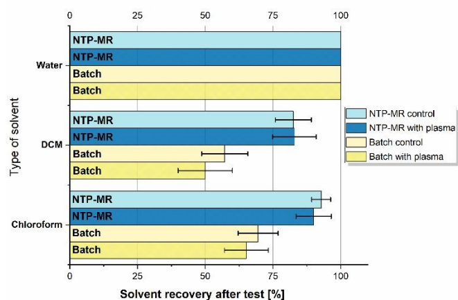
Figure 6 Percentage solvent recovery with exposure to gas flow only (control) and NTP (with plasma). Values shown on the graph represent the mean of 3 repeats, error bars represent standard error taken from repeated measurements ( n=3 ).
