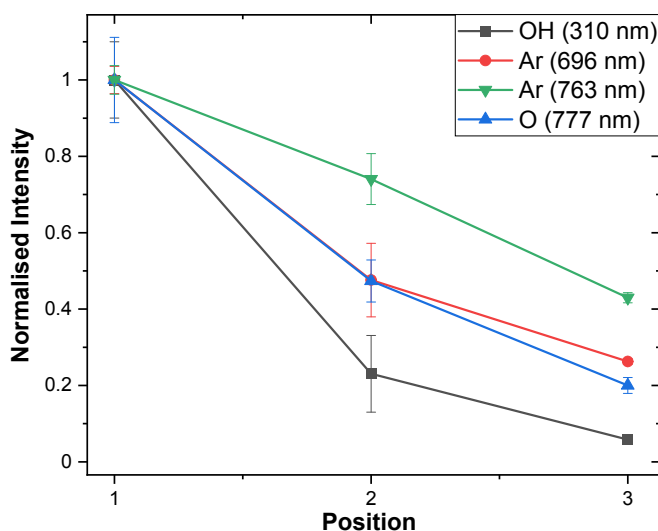
Figure 5 Normalised peak intensities of OH, Ar, and O species observed by OES at positions 1, 2, and 3 (Fig. 1). Error bars represent by standard error taken from repeated OES measurements ( n=3 ).
