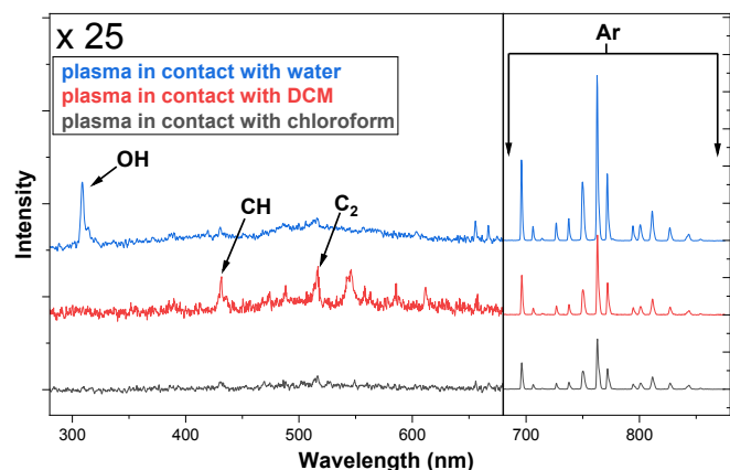
Figure 3 OES measurements of plasma glow in contact with three solvents, recorded at the junction in the microfluidic reactors (blue spot marked 1, Fig. 1).
