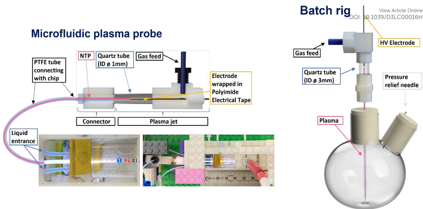
Figure 1 Schematic representation of microfluidic and batch NTP reactors. Numbers on the microfluidic chip indicate positions where OES was performed.
