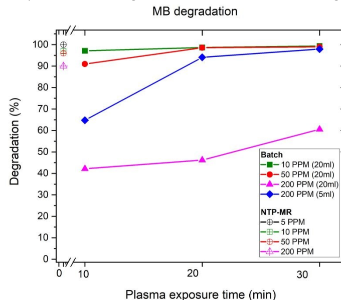
Figure 2 Plot of MB degradation percentage against plasma exposure time in batch and NTP-MR.
