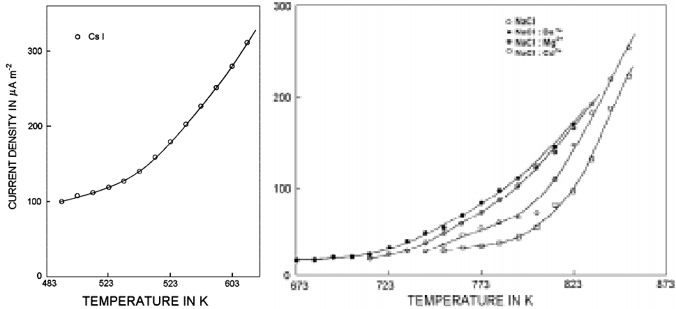
Fig. 1. Dependence of the current density on temperature for a constant injection field of 550 V/cm in a pure CsI crystal.
