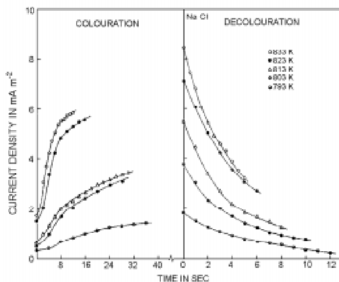
Fig. 3a. Dependence of the space-charge-limited current density on injection time for both colouration and decolouration at different temperatures in a pure NaCl crystal.
