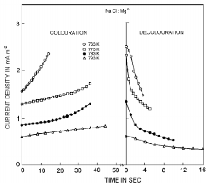
Fig. 3c. Dependence of the space-charge-limited current density on injection time for both colouration and decolouration at different temperatures in doped NaCl:Mg crystal.
