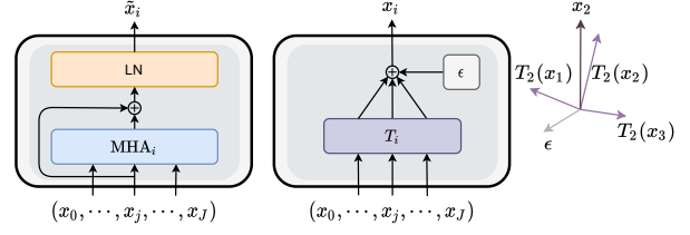
Figure 3: The self-attention block (left) at each position i can be decomposed as a summation of transformed input vectors (right). The closest vector ( T_2(x_2) ) contributes the most to \tilde{\mathbf{x}}_i .
