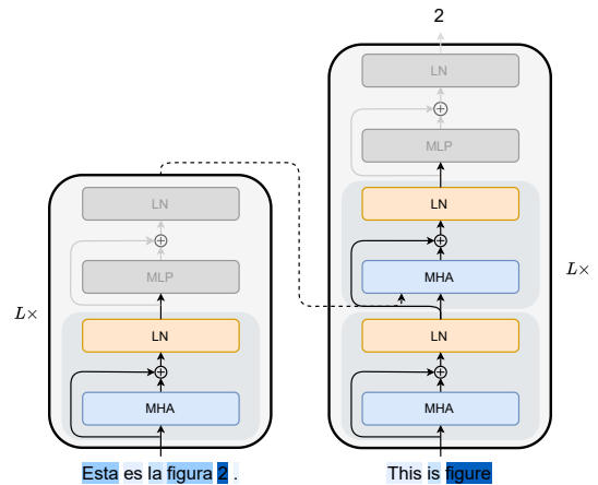
Figure 2: Encoder-Decoder Transformer.
