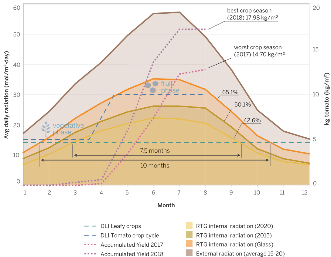
Fig. 5. Average daily solar radiation reached inside the greenhouse for the current polycarbonate material (S1.1, yellow/brown lines, measured in mol photons/ m^2 \cdot day ) according to monthly transmissivity values during the 2015–2020 period and the calculated solar levels reached for an AR-glass covering (S2.2, orange line). Accumulated tomato yields from the best and worst crop seasons (red-dotted lines) determine the vegetative and fruit phase of tomato plants and their respective daylight integral (DLI) needs (blue-dotted line).
