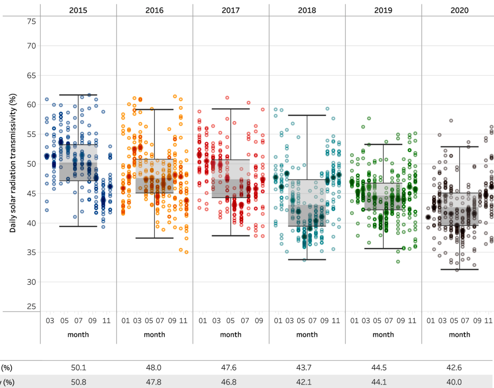
Fig. 4. Average daily (colored circles and table values), monthly (colored dots and box plots) and annual (box plots and table values) transmissivity values in the ICTA-iRTG SE (iRTG 1) recorded through iRTG internal and external global solar radiation sensors.
