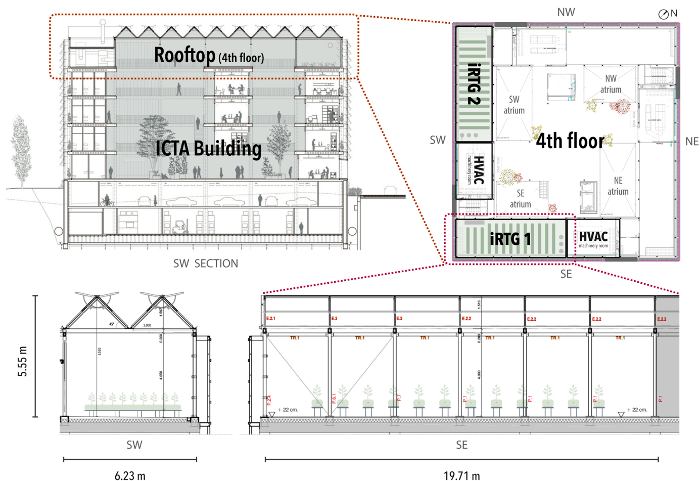
Fig. 1. ICTA-iRTG building SW section and floorplan distribution of the 4th floor including iRTG 1 geometry and SE, SW sections.
