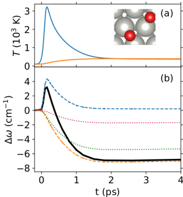
FIG. 1. Transient changes induced in CO/Pd(111) by a 450 nm pump pulse (100-fs duration and absorbed fluence of 40 \text{ J/m}^2 ) that hits the surface at t = 0.1 \text{ ps} . The initial temperature is 100 K. (a) Electron T_e(t) (blue) and lattice T_l(t) (orange) temperatures calculated with TTM. Inset: top view of the c(4 \times 2)\text{-}2\text{CO}_{\text{br}} unit cell. (b) Transient frequency shift of the CO IS mode: \Delta\omega(t) (black solid), \Delta\omega^{[1]}(t) (blue dashed), and \Delta\omega^{[2]}(t) (orange dashed). Contributions of the CO and surface phonons to \Delta\omega^{[2]}(t) are shown by red- and green-dotted lines, respectively.
