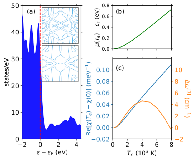
FIG. 2. (a) Electronic DOS of the CO/Pd(111) system. Vertical red dashed line marks the Fermi level. Insets: constant energy cuts of the band structure over the Brillouin zone at \epsilon = \mu(T_e) for T_e = 100 \text{ K} (top) and T_e = 3000 \text{ K} (bottom). (b) Dependence of the chemical potential with the electronic temperature. (c) Change in the real part of \chi (blue) and in \Delta\omega^{[1]} (orange) as a function of T_e .
