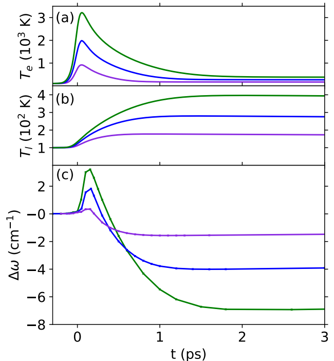
FIG. 3. Transient changes induced in CO/Pd(111) by a 450 nm pump pulse (100-fs duration) with different absorbed fluences: F = 6 (purple lines), 19 (blue lines), and 40 J/m 2 (green lines). The pulse maximum is at t = 0.1 ps and the system initial temperature is 100 K. (a) Electron temperature T_e(t) , (b) lattice temperature T_l(t) , and (c) transient frequency shift of the CO IS mode \Delta\omega(t) .
