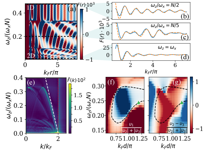
Figure 4. (a) Mediated potential F(r) as a function of the anisotropy ratio \omega_z/(N\omega_x) and effective atomic separation k_F r . Repulsive (attractive) forces are represented in red (blue). (b-d) Value of F(r) for three anisotropy ratios (blue) indicated in (a) with black dashed lines, compared to the expected analytic results (5,6) (orange). (e) Cosine transform of F(r) as a function of \omega_z/(N\omega_x) , where the dotted lines correspond to the frequencies 2k_F (red) and \tilde{k}_1 (white). (f,g) Relation between the nearest-neighbor potentials v_{1,2,3} of a kagome lattice with lattice spacing d , as a function of \omega_z/(\omega_x N) and k_F d . Dashed contour follows v_1 = 0 . Here we took N = 250 and the rest of the parameters as in Fig. 2.
