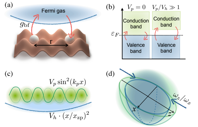
Figure 1. (a) Two bosonic atoms (white) separated by distance r and trapped in an optical lattice (red) experience an effective long-range interaction mediated by a Fermi gas trapped in an harmonic potential (blue). (b) The contact Bose-Fermi interactions ( g_{bf} ) virtually populates the conduction band of the Fermi gas. (c) An additional oscillatory potential induces a gap between the valence and conduction gap, exponentially damping the mediated interactions. (d) By controlling the strength of the trapping potential in an orthogonal direction, \omega_z/\omega_x , one can continuously tune the dimension of the Fermi gas from 1D to 2D, introducing additional modulating frequencies as will be shown in Fig. 4.
