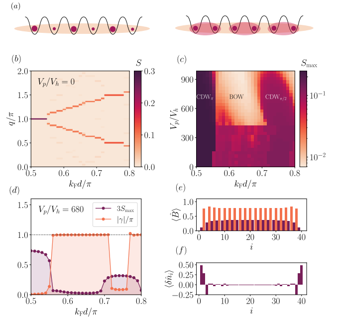
Figure 3. (a) Real-space configuration of the \text{CDW}_\pi (left), where spheres of different sizes correspond to an alternating atomic occupation, and frustrated BOW (right) with a dimerized bond structure. (b) S(q) as a function of k_F d for a chain with L = 60 sites and bosonic density \rho = 1/2 , for V_p = 0 . The phase diagram presents a staircase structure, where every step corresponds to a \text{CDW}_q characterized by a peak in S(q) . (c) Value of S at the peak, S_{\text{max}} as a function of k_F d and V_p/V_h , showing how the CDW orders melt for sufficiently large values of V_p/V_h , giving rise to a frustrated BOW. (d) S_{\text{max}} and Berry phase \gamma as a function of k_F d for V_p/V_h = 680 , showing the non-trivial topological nature of the BOW phase. Real-space configuration of the BOW phase for L = 40 , showing (e) dimerized bonds and (f) localized edge-states at the boundaries. Parameters as in Fig. 2.
