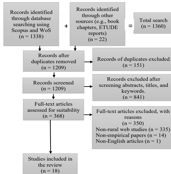
Figure 2. Flowchart of the selection procedure.
