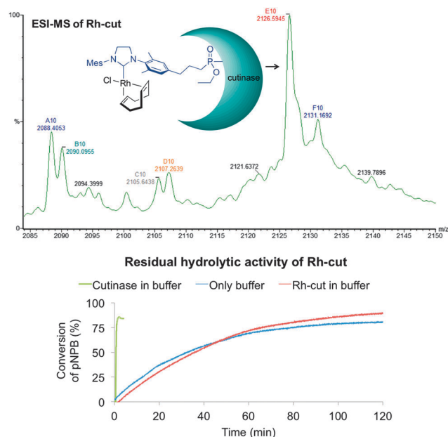
Fig. 1 ESI-MS analysis of Rh-cut hybrid (top, [\text{M}]^{10+} calc.: 2127.43, found: 2126.59) and the determination of residual hydrolytic activity of cutinase (bottom).
