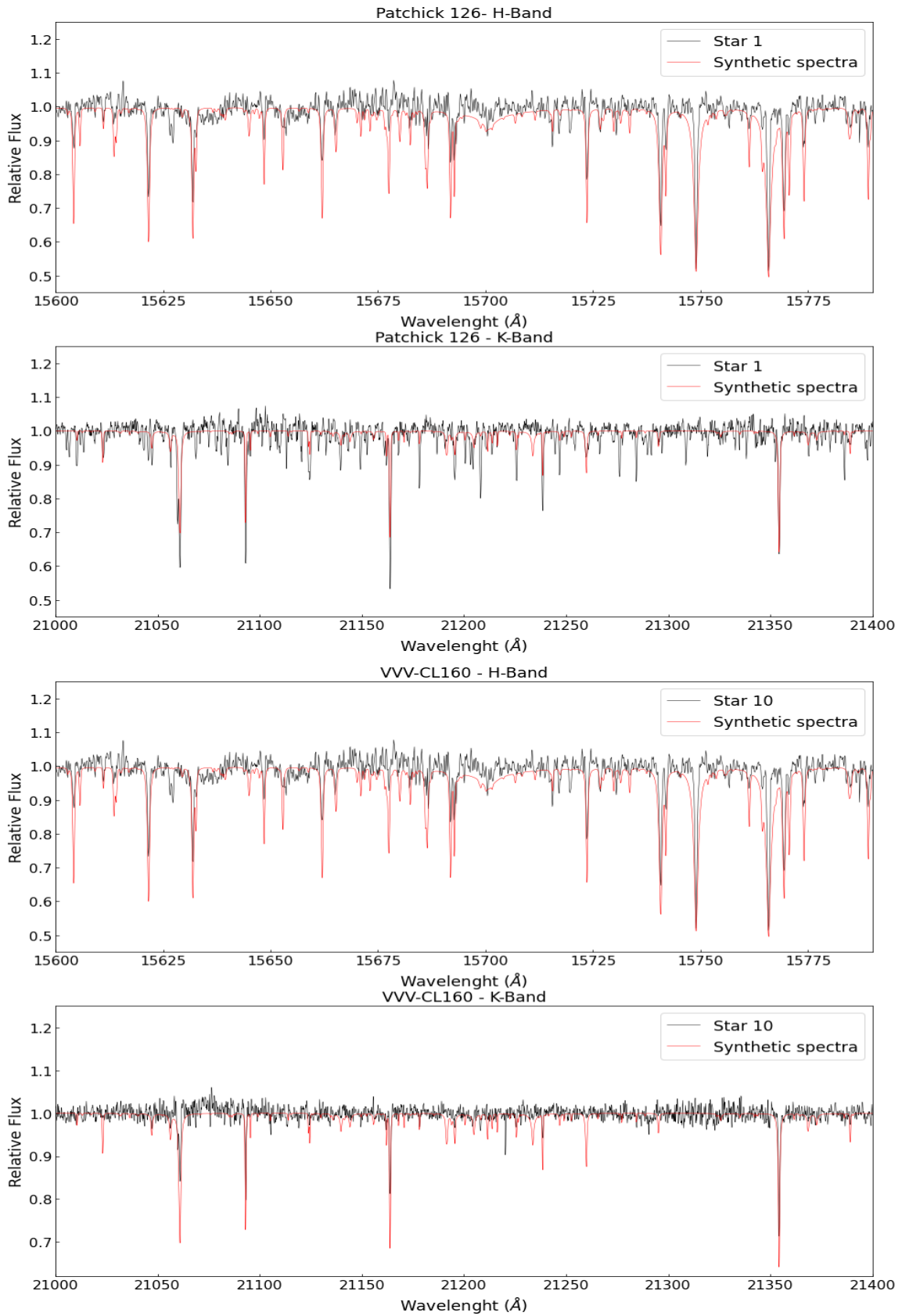
Fig. 3. Cross-correlation. Representative IGRINS H - and K -band spectra of two RGB stars: Star 1 for Patchick 126 and Star 10 for VVV-CL160 (black lines). We superimposed the synthetic solar spectra (red lines) used for determination of cross-correlation velocities in the spectral regions between 15 000 and 17 000 \text{\AA} in the H -band, and between 19 500 and 22 900 \text{\AA} in the K -band.
