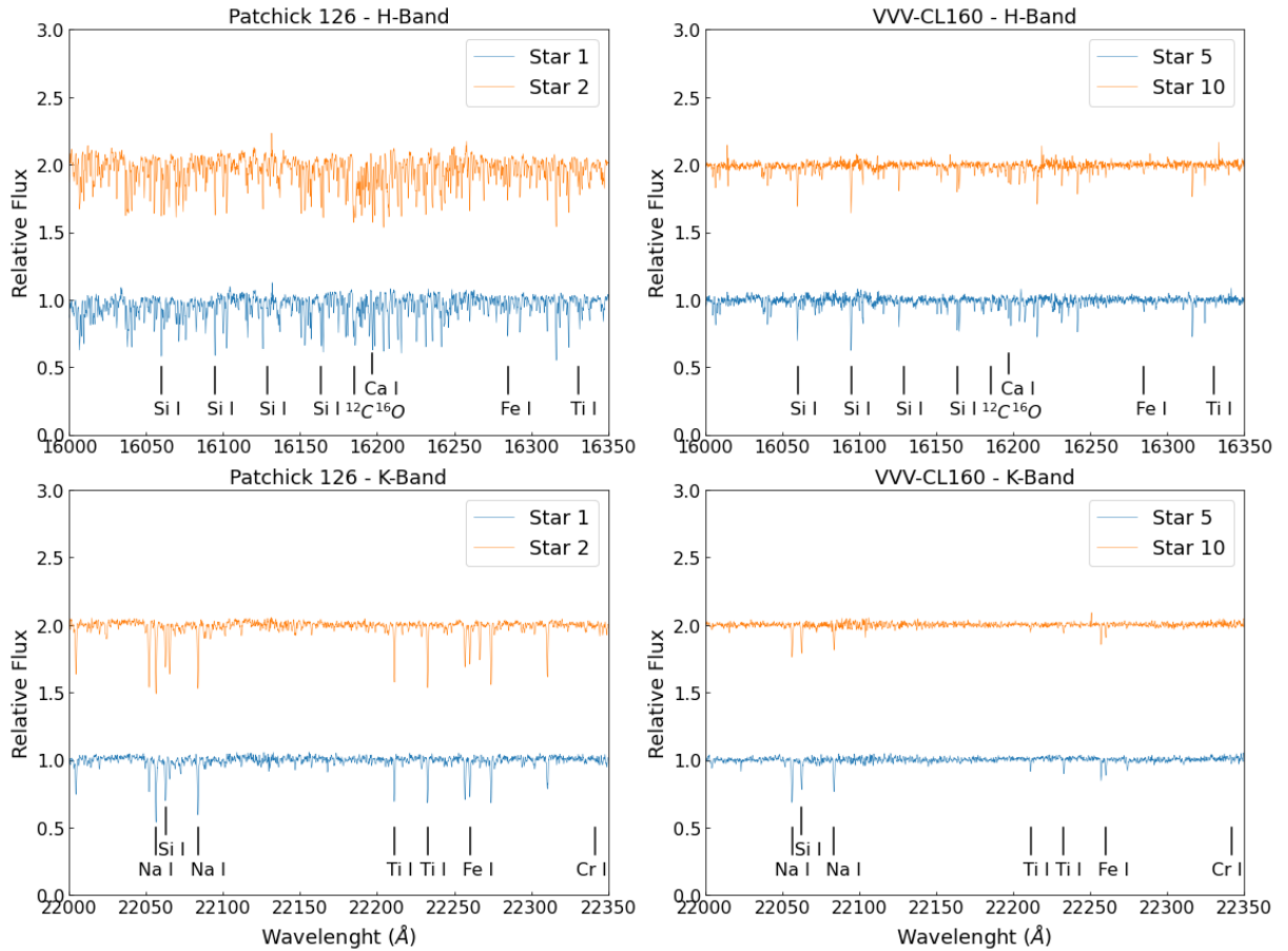
Fig. 1. Final IGRINS spectra. Representative IGRINS H - and K -band spectra of two RGB stars in each GC in air wavelengths: Star 1 and Star 2 for Patchick 126 (left panels), and Star 5 and Star 10 for VVV-CL160 (right panels). For clarity in the plot, we have shifted the relative flux scale of Star 2 and Star 10 vertically with additive constants, and show zoomed spectra between 16 000 and 16 350 Å in the H -band and between 22 000 and 22 350 Å in the K -band. We identified some spectral features (Si I, Ca I, Na I, Fe I, Ti I and C 12 O 16 ).
