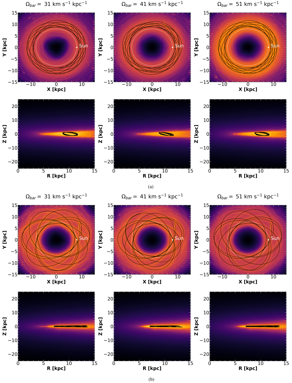
Fig. B.1. Orbits. Ensemble of 10 000 orbits for each studied star cluster by considering the errors on the observables, projected on the equatorial (top panels) and meridional (bottom panels) Galactic planes in the inertial reference frame, with a bar pattern speed of 31, 41, and 51 km s -1 and integrated over the past 2.0 Gyr. The red and orange colours correspond to more probable regions of the space, which are crossed most frequently by the simulated orbits. The black line shows the orbit of the star cluster from the observables without error bars. (a) ESO 92-18. (b) Ferrero 54. (c) Gaia 2. (d) Kronberger 99. (e) Kronberger 119. (f) Kronberger 143. (g) Patchick 122. (h) Patchick 125. (i) Patchick 126. (j) ESO 98-3. (k) VVV-CL60.
