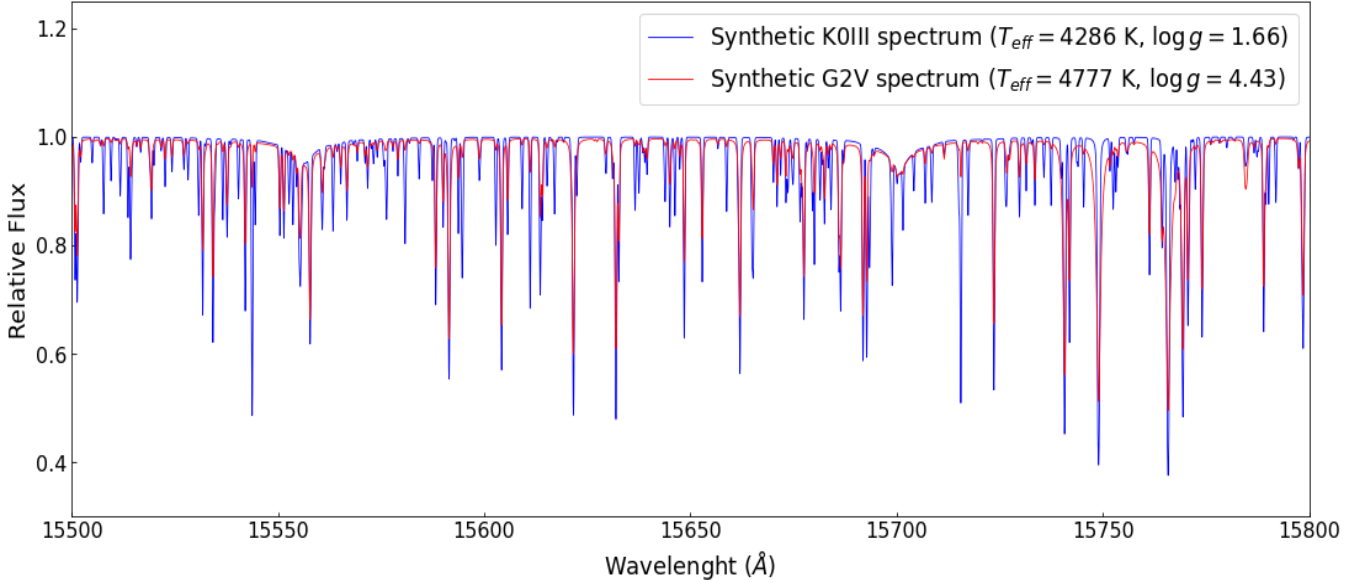
Fig. 2. Synthetic spectra. Comparison between spectra for Arcturus and the Sun.
