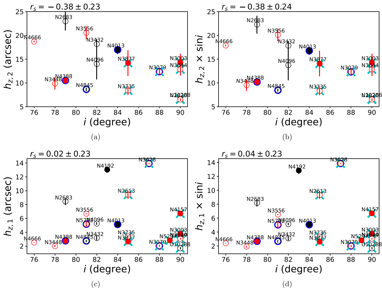
Figure 3. Comparison of the H \alpha scale heights in (a) component 2 (thick) and (c) component 1 (thin) with the inclination angles ( i ). Panels (b) and (d) show scale heights that have been modified by multiplying with \sin i in order to check the effect of inclination.
