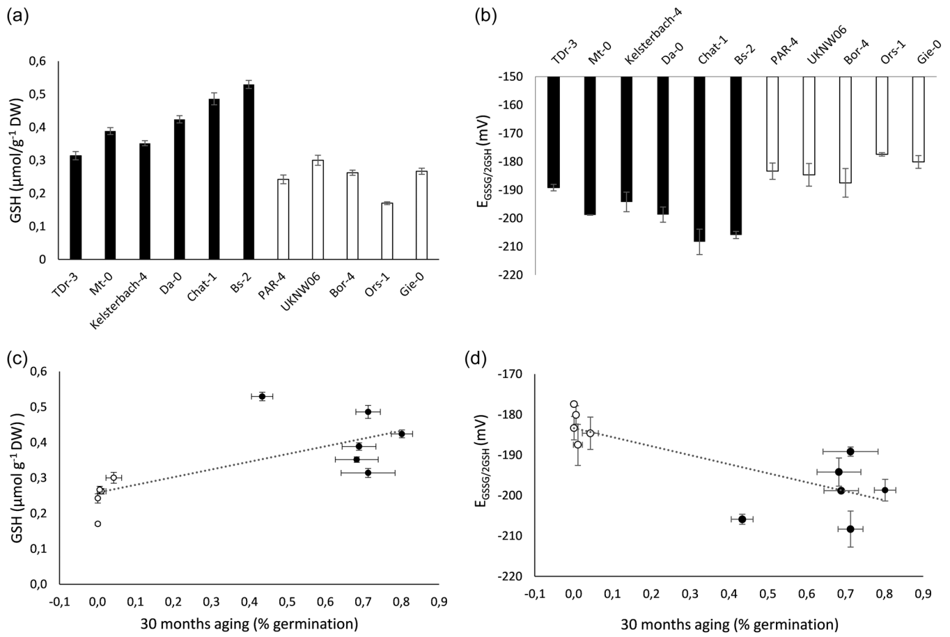
FIGURE 9 Relationship between glutathione and seed longevity in Arabidopsis wild-type accessions. (a) Concentrations of glutathione (GSH) and (b) glutathione half-cell reduction potentials ( E_{GSSG/2GSH} ). Reflecting cellular redox state in dry seeds. Data are means of four replicates \pm SD. (c, d) Correlation of data shown in (a) and (b), respectively, with total germination after 30 months of ambient ageing
