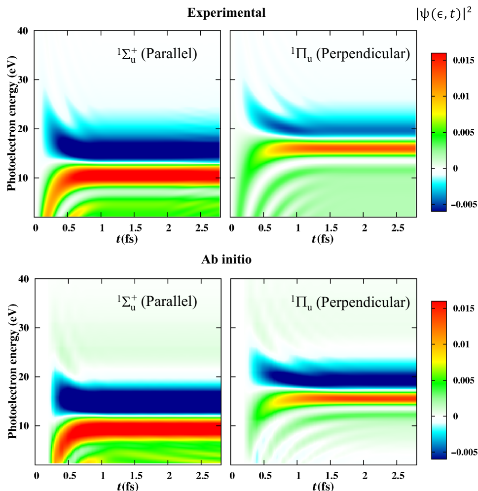
Fig. 3. Buildup in time of the interference between direct ionization and autoionization from the lowest Q_1 1\Sigma_u^+ (left panels) and Q_2 1\Pi_u (right panels) doubly excited states corresponding to the v = 5 vibrational state of the remaining H_2^+ ion. Similar plots can be obtained for other final v s. (Top) Square of the wave packet densities obtained from experiment as a function of photoelectron energy (y axis) and time (x axis). (Bottom) Results of the ab initio calculations for a pulse of 200 as. For a better visualization, the monotonic decreasing background associated with the direct ionization channel has been subtracted in all cases.
