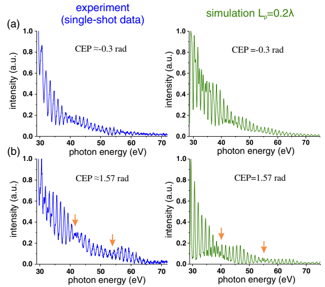
Fig. 8. XUV spectra for different CEP values: single-shot experimental results (left panels) and line-outs of simulation (right panels). (a) Case with the smallest modulation depth and best isolation degree [cf. Fig. 9(d) and the main text for details]. (b) Case with a pronounced beating structure (beating nodes are marked with arrows), which corresponds to the generation of three attosecond pulses with nearly equal amplitudes.
