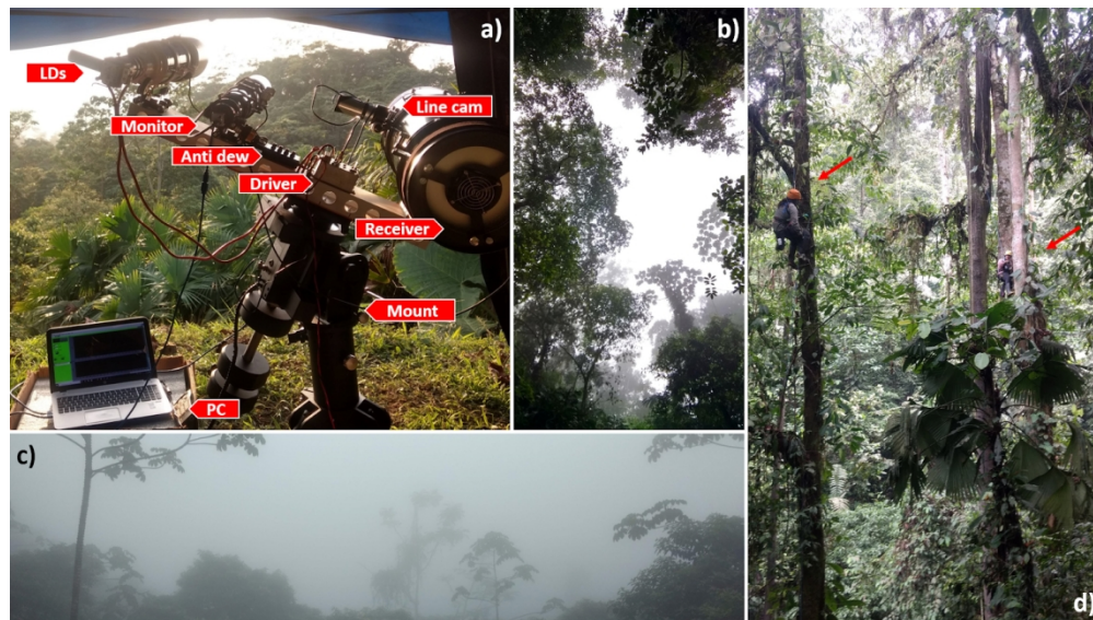
Fig. 1. a) Entomological-lidar system and its main components overlooking the Jardin de los sueños private forest, during a clear moment (17:30). b) Photo displaying the top of canopies at \sim 30 m over ground disappearing into the mist (9:30), c) A view from lidar toward valley at noon (12:05), typical of the field campaign days. The mist is impenetrable. d) Ecological studies in tropical virgin forests are challenging due to topography, tall vegetation structure, and stratification of ecological niches, here two chiroptologists install a bat net 20 m above ground.
