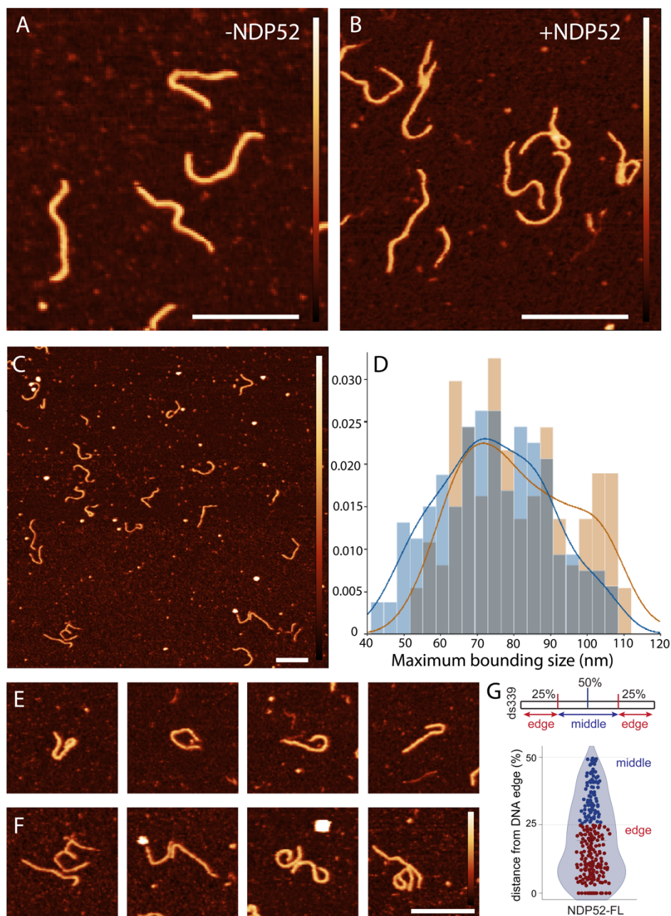
Figure 6: NDP52 changes DNA conformation in vitro . (A) AFM image of ds339 on PLO in the absence of NDP52. Scale bar = 100 nm. Height scale = 4.5 nm (B) AFM image of ds339 on PLO with NDP52. Scale bar = 100 nm. Height scale = 4.5 nm. (C) AFM images of NDP52-FL bridging strands of linear (339 bp) dsDNA on poly-L-ornithine surface. Scale bar = 100 nm. Height scale = 4.5 nm (D) Normalised histogram comparing the maximum bounding size of DNA with (light blue) and without NDP52 (orange); their distributions overlap (dark blue). (E) Cropped AFM images of DNA molecules in the presence of NDP52 on PLO. First two images are from between 50- 60 nm maximum bounding size while the second two are between 80 - 90 nm. (F) AFM images showing bridging between DNA molecules in the presence of NDP52 on PLO. xy scale bars 100 nm. (G) Preference for NDP52-FL binding on ds339 molecule. Diagram shows ds339 edge and middle references on linear DNA. Violin plot shows %distance from DNA edge values for NDP52-FL binding. Mean \pm SEM is shown for n=270 binding events.
