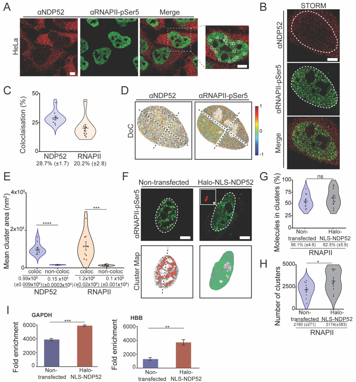
Figure 7: Colocalisation of NDP52 with RNAPII-pSer5. (A) Immunofluorescence confocal image of NDP52 (red) and RNAPII-pSer5 (green) in HeLa cells, showing detail of colocalising foci in white circles (zoomed-in right panel). Scale bar = 5µm (B) Example STORM images of NDP52 and RNAPII-pSer5 in HeLa. The nuclear region (determined by RNAPII-pSer5 fluorescence) was used for ClusDoC analysis (shown as dotted white line). Scale bar = 5µm (C) Colocalisation analysis of NDP52 and RNAPII-pSer5 clusters (n = 10 cells Errors bars are mean ± SEM). (D) Cluster colocalisation heat maps for NDP52 and RNAPII-pSer5 generated from the STORM data shown in (B). DoC score of 1 represents perfect colocalisation between molecules, and DoC score -1 represents segregation. A DoC score of 0.4 was used as threshold for colocalisation. Due to high molecular density the nucleus was split into four ROIs for ClusDoC analysis. Axis of separation for the images are shown as dotted lines. (E) Mean cluster area is shown for colocalised and non-colocalised clusters of NDP52 and RNAPII-pSer5. n = 10 cells. Errors bars are mean ± SEM. (F) STORM rendering for RNAPII-pSer5 and generated cluster maps for HeLa cells non-transfected or transiently expressing a Halo-NLS-NDP52 construct. Inset in Halo-NLS-NDP52 panel shows wide-field channel Halo ligand-JF549 labelled cells. Scale bar = 5µm. (G) Percentage of RNAPII-pSer5 molecules in clusters
