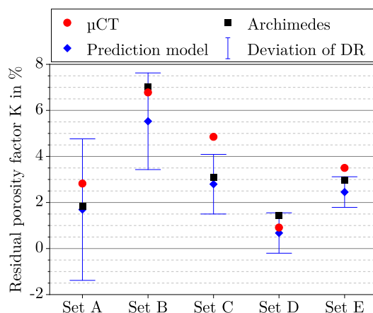
Figure 10. Comparison of the three residual porosity factors determined theoretically and experimentally for the parameter sets from Table 2. Set A = LT150DAR14DR32, Set B = LT200DAR11DR45, Set C = LT200DAR14DR75, Set D = LT200DAR17DR113, and Set E = LT250DAR14DR147. The abbreviation \mu CT and Archimedes refers to the two experimental methods. The error bar includes the model prediction in case of a statistical deviation of the DR by an absolute of 1%.
