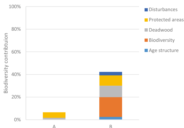
Fig. 13 Results of two case study scenarios, where A represents intensive management practices and B are less intensive management practices. Higher values represent a higher contribution to biodiversity, i.e., a more preferable situation
