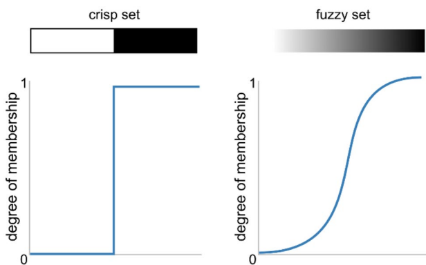
Fig. 2 Illustration of crisp and fuzzy sets and membership functions
