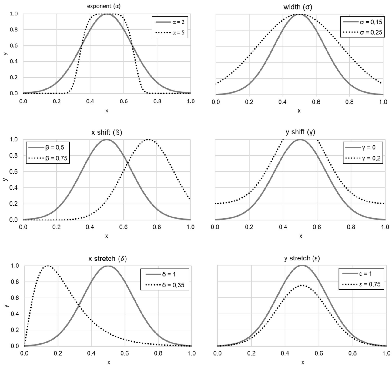
Fig. 4 Examples of Gaussian curve with altered constants \alpha , \sigma , \beta , \gamma , \delta , and \epsilon
