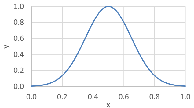
Fig. 3 Gaussian distribution, or basic function
