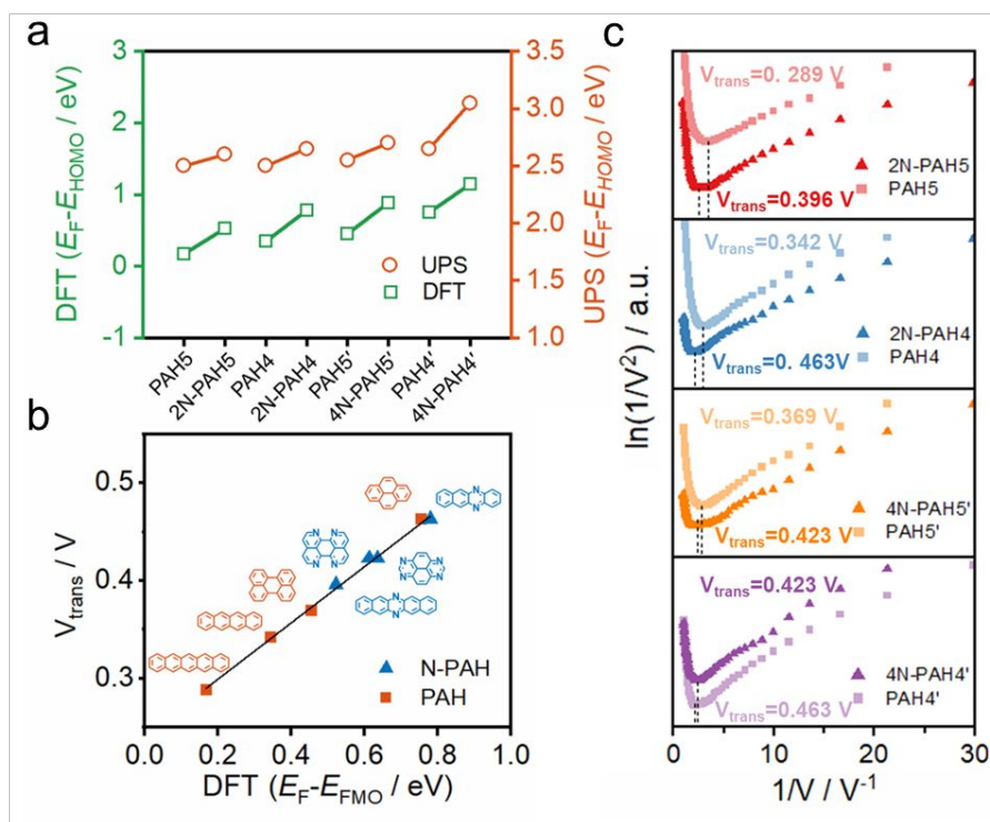
Fig. 3 Ultraviolet photoelectron spectroscopy and transition voltage spectroscopy. (a) Comparison of E_F - E_{\text{HOMO}} by UPS with E_F - E_{\text{FMO}} by DFT theoretical calculation. (b) V_{\text{trans}} versus E_F - E_{\text{FMO}} by DFT theoretical calculation difference. (c) The transition voltage ( \ln(I/V^2) vs 1/V ) spectra were obtained by over 500 I - V traces of 2N-PAH5, PAH5, 2N-PAH4, PAH4, 4N-PAH5', PAH5', 4N-PAH4', PAH4'.
