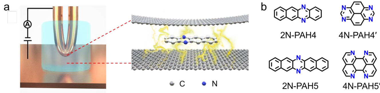
Fig. 1 Schematic diagrams and molecular structures. (a) Schematic diagrams of the cross-plane break junction (XPBJ) setup based on STM-BJ setup (left) and the structures of sandwiched molecular junctions with a N-PAH (right). (b) Chemical structures of N-PAHs, including 5,12-diazatetracene (2N-PAH4), 1,3,6,8-tetraazapyrene (4N-PAH4'), 6,13-diazapentacene (2N-PAH5), 1,6,7,12-tetraazaperylene (4N-PAH5').
