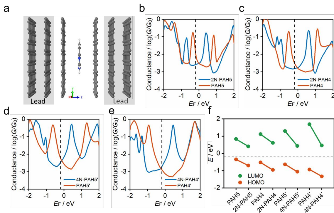
Fig. 4 Electrical conductance properties of graphene-molecule-graphene van der Waals heterojunctions. (a) Structure of sandwiched molecular junctions with a 4N-PAH4' molecule. (b-e) The electrical conductance of N-PAHs and PAHs molecules as a function of Fermi energy. The black dashed line ( E_F = -0.18 eV) shows the Fermi energy that agrees with the experiment results. (f) Energetic position of HOMO and LUMO resonances of graphene-molecule-graphene junctions obtained from Fig. b-e. The black dashed line shows E_F = -0.18 eV.
