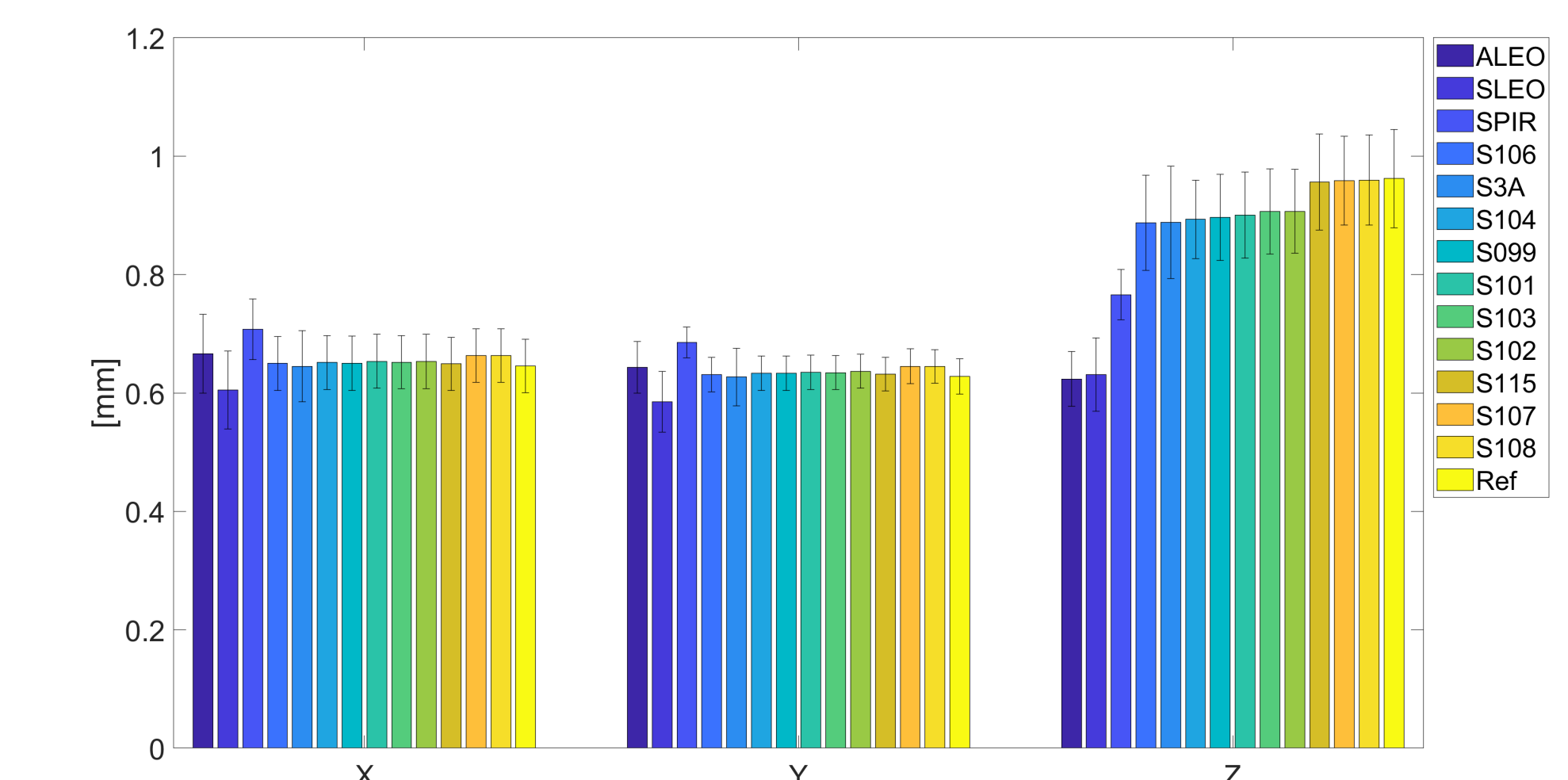
Figure 4: Formal errors Earth's center-of-mass estimates
