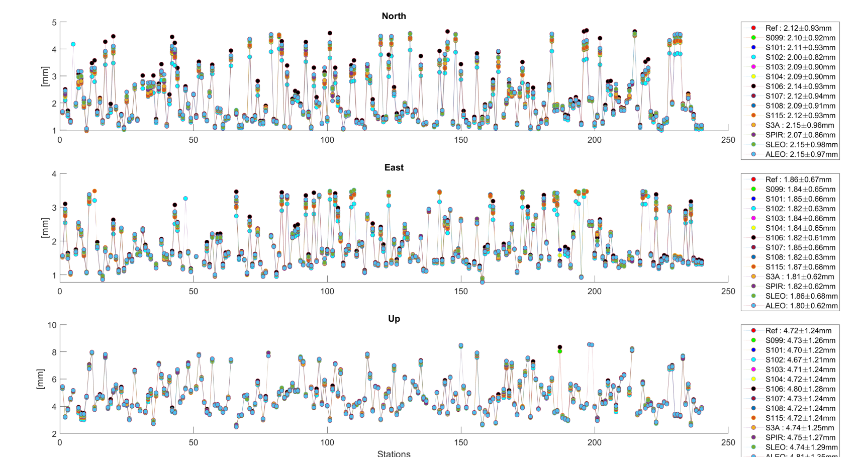
Figure 6: Repeatability of ground station coordinates
