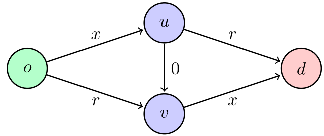
Figure 2. (Color online) The Network of Example 1
