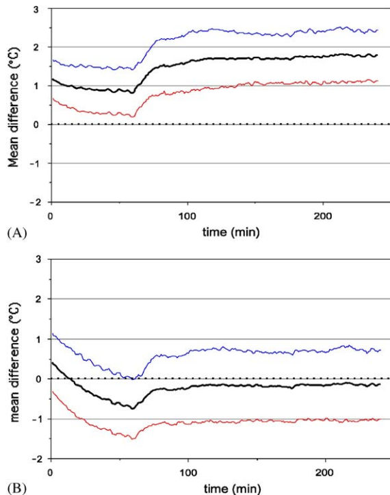
Fig. 1. (A) Mean difference (bold line) with SD (thin line) between modeled and measured skin temperature plotted against time, using the standard subject in the model (B) and with input in the model of subject characteristics and actual measured MR.
