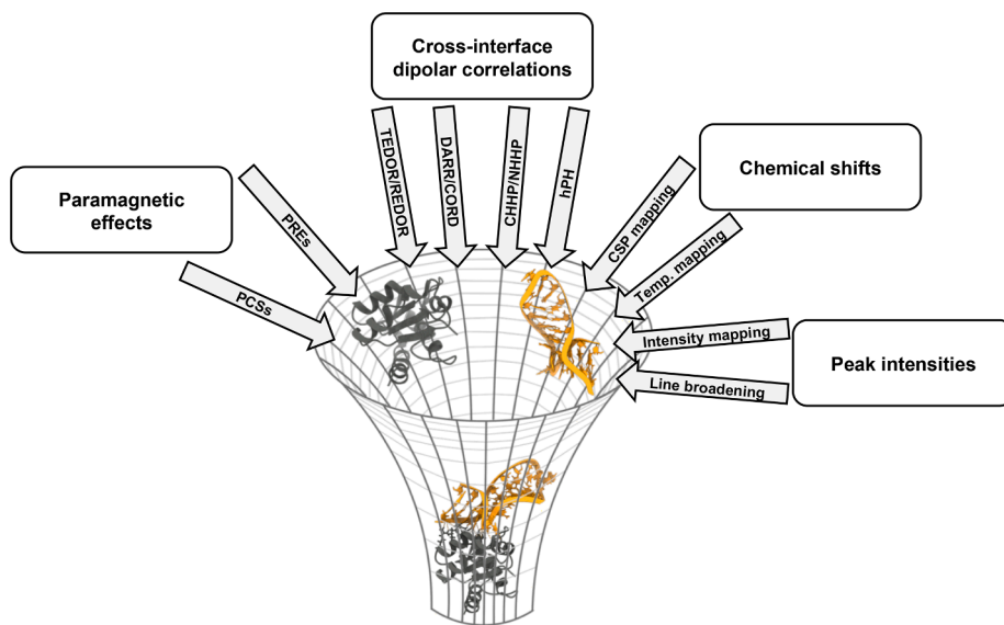
Fig. 2. Overview of ssNMR methods utilized to date to probe nucleic acid–protein interfaces. Information derived from paramagnetic effects, cross-interface dipolar correlations, chemical shifts and peak intensities are highly complementary and can be utilized as restraints in a molecular docking protocol that builds the nucleic acid–protein complex from the structures of the individual components. Pseudo contact shifts (PCSs) measure changes in chemical shifts due to the influence of a paramagnetic ion with anisotropic tensor. Paramagnetic relaxation enhancement (PRE) measures the increase in relaxation of nuclei in the vicinity of an unpaired electron. Both effects can be quantified and translated into nucleus–electron distances. Cross-interface dipolar correlations directly measure intermolecular distances through a variety of dipolar recoupling techniques. The ssNMR toolbox for the measurement of intermolecular distances covers transferred echo double resonance (TEDOR)/ rotational echo double resonance (REDOR)-based recoupling experiments, ^{13}\text{C} – ^{13}\text{C} correlation experiments, such as dipolar assisted rotational resonance (DARR) and combined \text{R}2_n^v -driven (CORD), spin-diffusion based CHHP/NHHP experiments, and ^1\text{H} -detected CP-based hPH experiments. Chemical shift perturbation (CSP)
