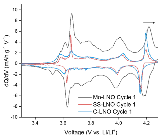
Figure 4- Comparison of first cycle differential capacity (dQ/dV) plots for Mo-LNO (black), SS-LNO (red) and C-LNO (blue) in the voltage window 2.7-4.3 V. This shows a shift to a higher voltage for the H2-H3 phase transition in Mo-LNO.
