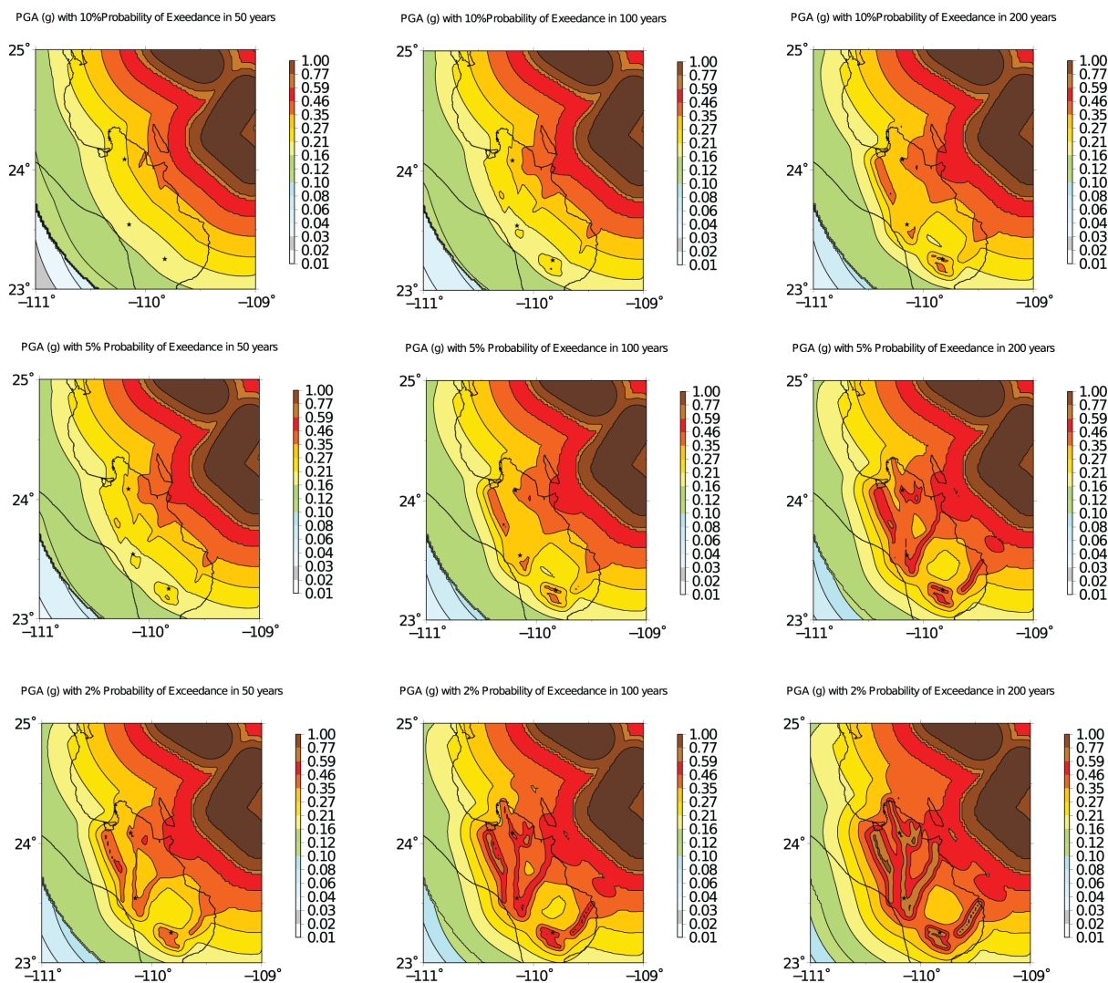
Figure 6. Probabilistic seismic hazard analysis for different return periods and observation times using the WSJ model. The transform fault system is located at the top right of the map and it was analyzed with the Gutenberg-Richter model. The Quaternary faults are located within the Baja California Peninsula and analyzed with the Characteristic model (see text for details).
