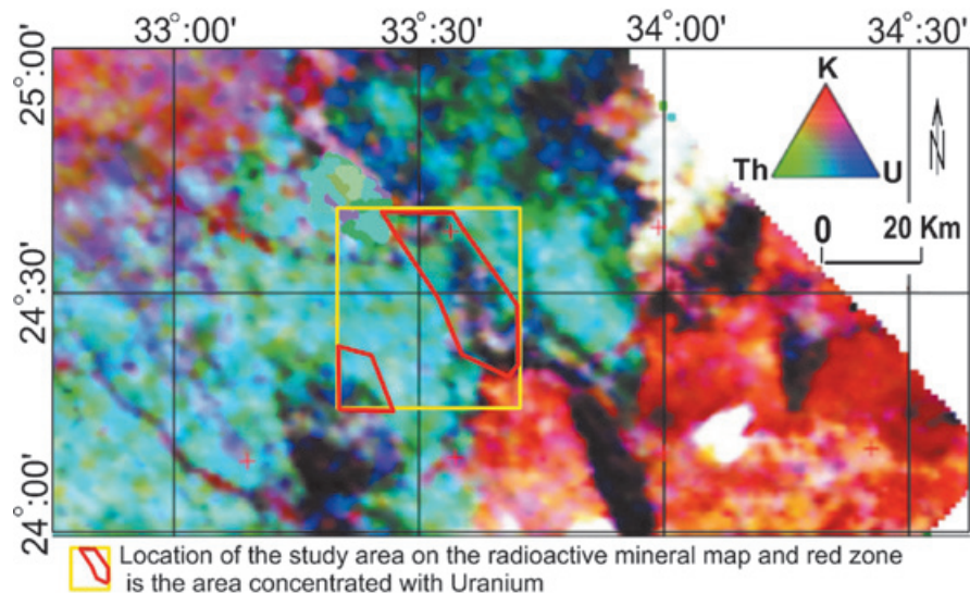
Figure 8. Radioelement composite image (after Elawadi et al. 2004) showing zones with radioactive mineral accumulations.
