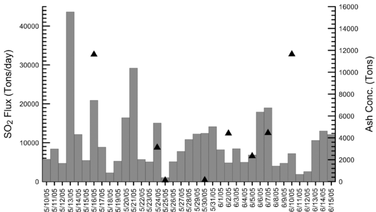
Figure 5. Ash concentration (black triangle) and SO 2 flux emissions (bars) obtained by MODIS retrievals.
