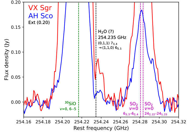
Fig. C.2. Emission line profiles toward AH Sco (blue) and VX Sgr (red) in the vicinity of the v = 0 , J = 6-5 transition of ^{30}\text{SiO} (at 254.217 GHz) and of the (0,1,1) 7_{3,4}-(1,1,0) 6_{5,1} transition of para water near 254.235 GHz (line 9, Table 2). The spectra are extracted from the high resolution data for a circular aperture of 0''.2 diameter and plotted in the rest frequency frame. The dotted black vertical line is the expected water frequency according to Furtenbacher et al. (2020) (see Table 2). Identification of the water transition at 254.235 GHz is uncertain (see discussion in Appendix C).
