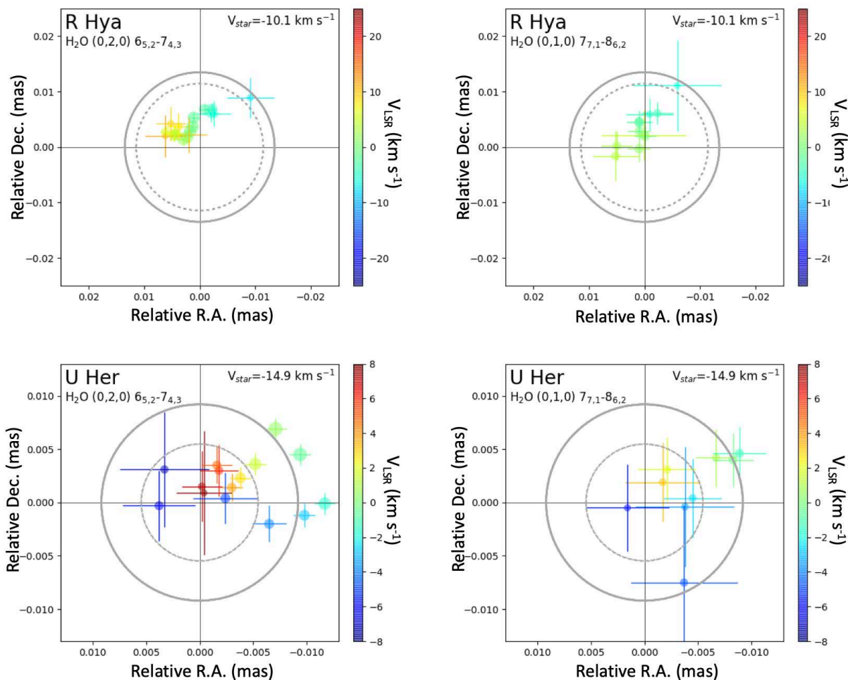
Fig. 10. Maps of the different velocity components of water identified in the Gaussian-fit procedure at 268.149 and 262.898 GHz toward R Hya and U Her for the extended configuration of the main array. The size of the colored symbols varies as the square root of the integrated flux density of the Gaussian component; the crosses show the position uncertainty for each component. The velocity scale colors are given on the right side of each map with respect to the stellar system velocity taken to be -10.1 and -14.9 \text{km s}^{-1} in the LSR frame for R Hya and U Her, respectively. The dashed gray circle represents the size of the optical photosphere (23.7 and 11.2 mas for R Hya and U Her, respectively) and the larger gray circle represents the 250 GHz continuum emission size (27.1 and 18.5 mas for R Hya and U Her).
