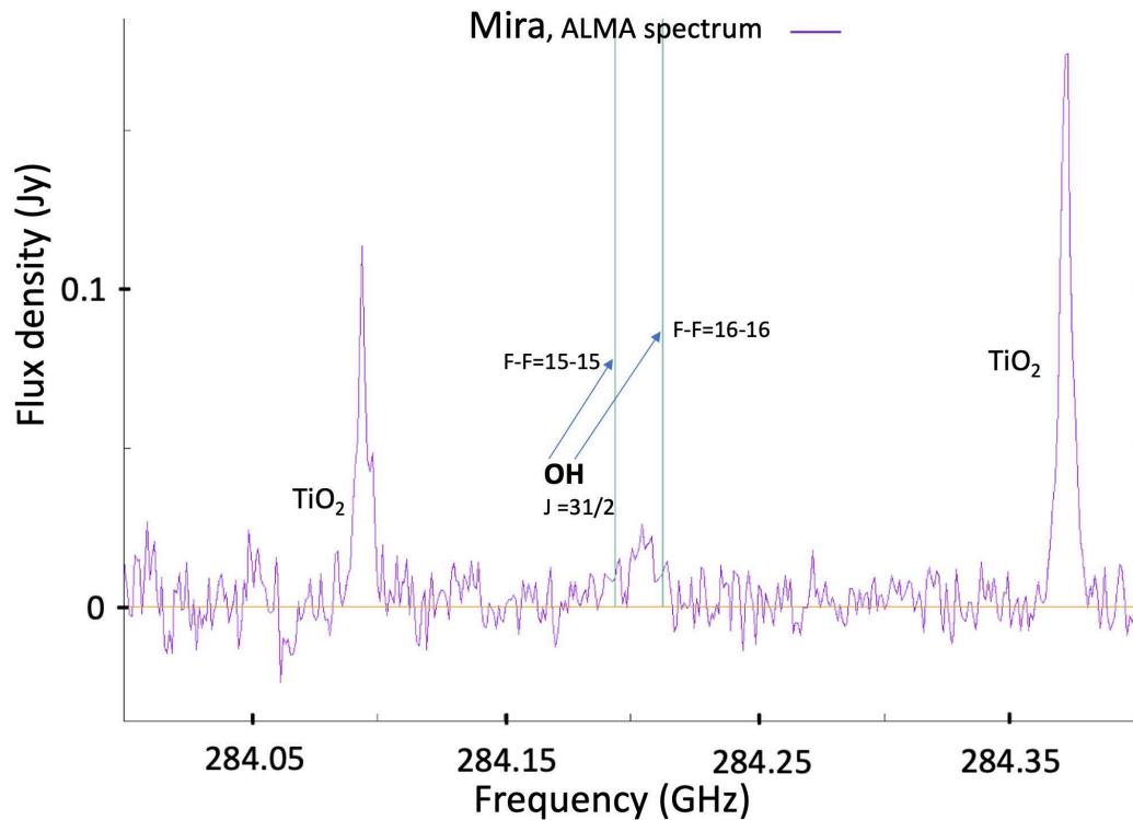
Fig. F.2. Line spectrum in the vicinity of the \nu = 0 , J = 31/2 rotational level of OH and of two nearby TiO 2 transitions observed in the 284.00 to 284.40 GHz range toward omi Cet (Mira). The expected F' - F'' = 15 - 15 and 16 - 16 hyperfine transitions of OH in the J = 31/2 \Lambda -doublet are indicated with two light green vertical lines at the expected frequencies. The two TiO 2 lines correspond to the 27(7, 21) - 27(6, 22) and 21(1, 21) - 26(0, 20) transitions at 284.0943 and 284.3719 GHz, respectively. Spectrum extracted from a 0''.25 \times 0''.20 region containing all the OH emission.
