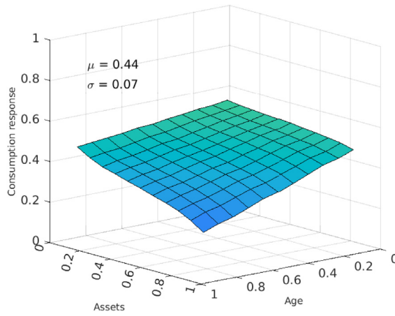
Fig. D.22. Average consumption responses to labor income. Notes: PSID, 2005–2017 sample, dual earners, labor income. The graph shows the average derivative of log-consumption with respect to the persistent latent component \eta_{it} in a model without unobserved heterogeneity \xi_i in consumption. The two horizontal axes show age and assets percentiles, respectively.
