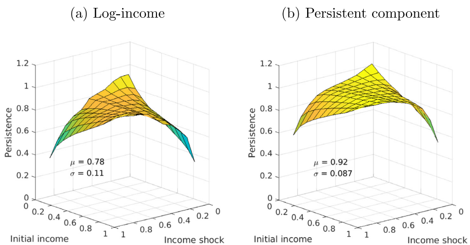
Fig. D.2. Nonlinear income persistence. Notes: PSID, 2005–2017 sample, disposable income, dual earners from an alternative perspective. The left graph shows quantile derivatives of log-income with respect to lagged log-income. The right graph shows quantile derivatives of the persistent latent component \eta_{it} with respect to \eta_{it-1} , model estimated using sequential Monte Carlo with a stochastic EM algorithm. The two horizontal axes show percentiles of \eta_{it-1} (“initial income”) and conditional percentiles of \eta_{it} given \eta_{it-1} (“income shock”), respectively.
